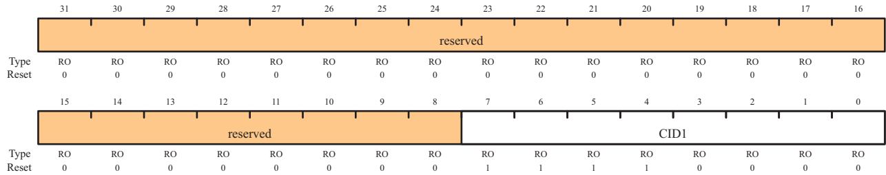
UART Primecell Identification 1 (UARTPCelIID1)
