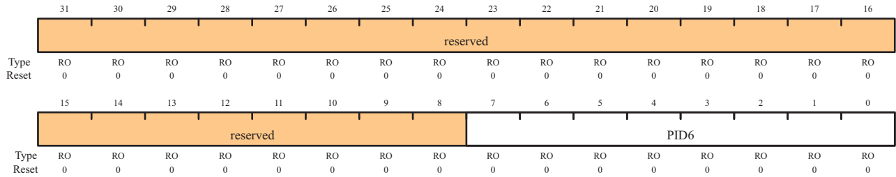
SSI Peripheral Identification 6 (SSIPeriphID6)
