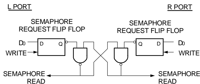
Figure 4. IDT70T16/5 Semaphore Logic
