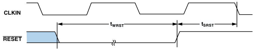
Figure 6. Reset
