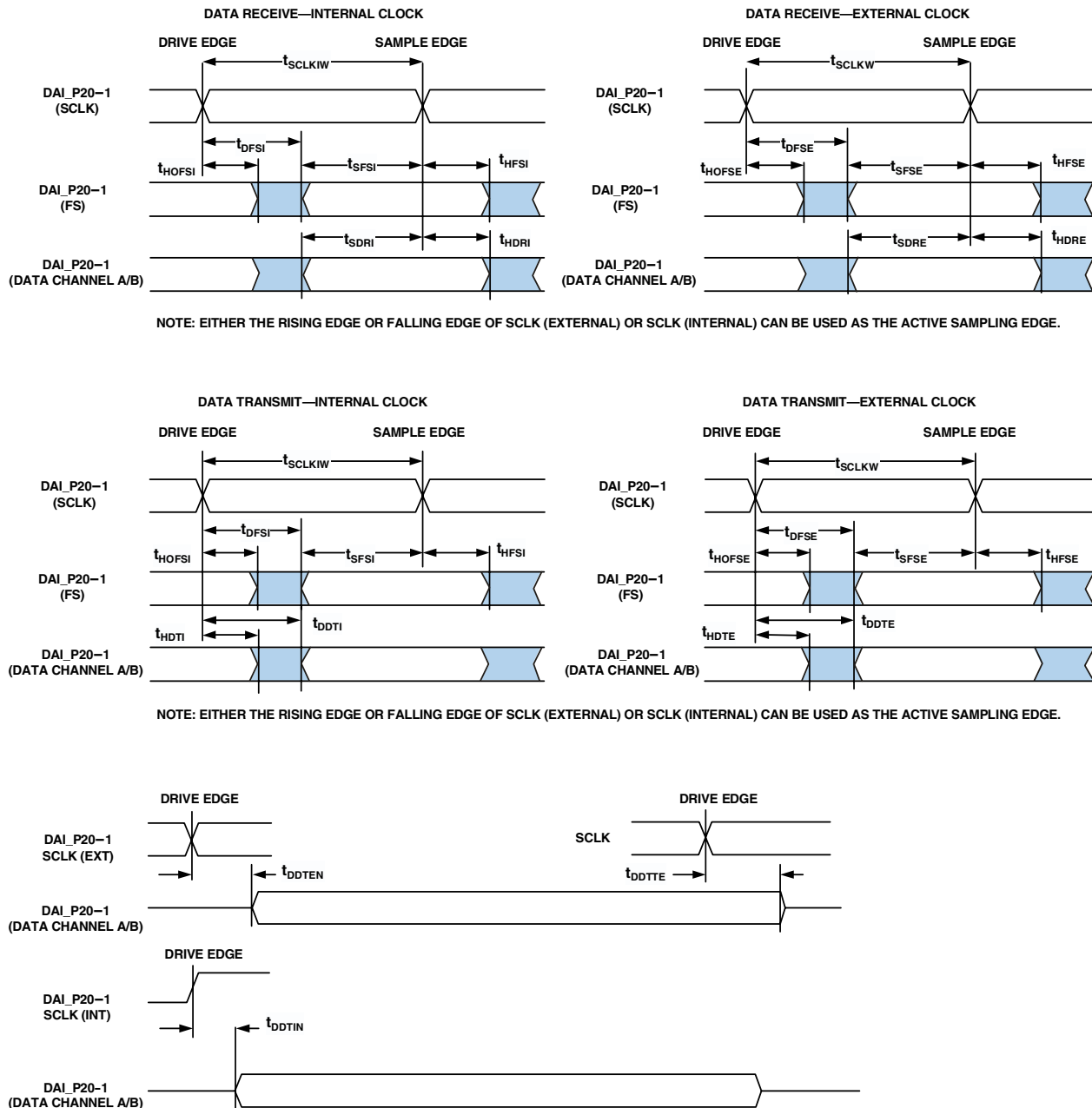
Figure 17. Serial Ports
