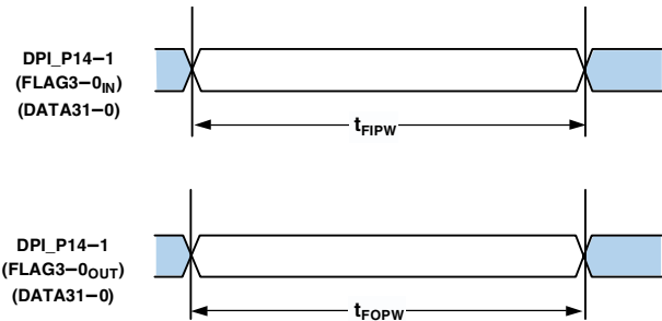
Figure 12. Flags
