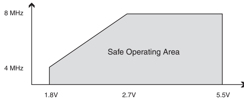
Figure 26-2. Maximum Frequency vs. V_{CC} , ATmega165PV
