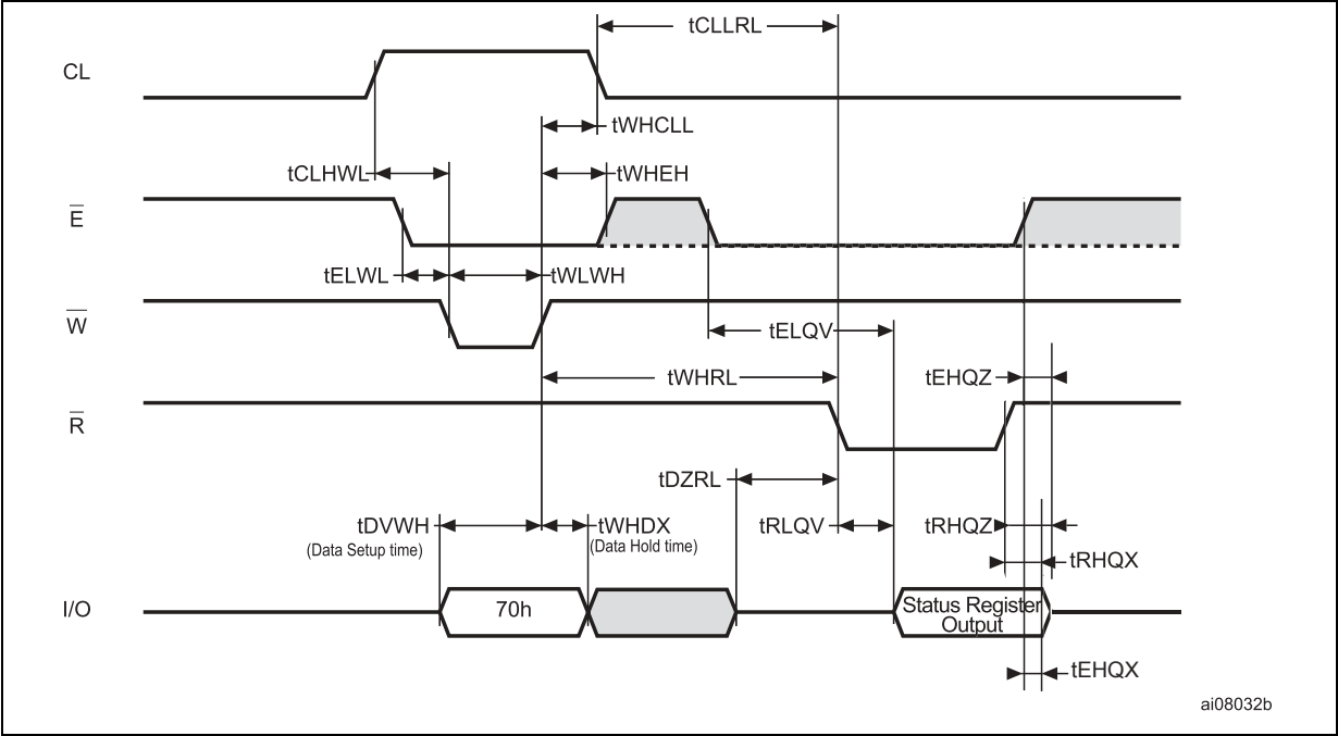
Figure 21. Read Status Register AC waveforms
