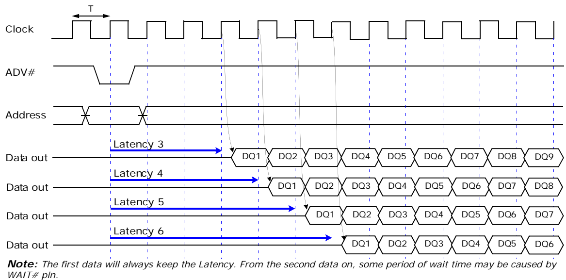
Figure 41.1 Latency Configuration (Read)
