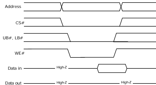
Figure 39.2 Asynchronous Write
