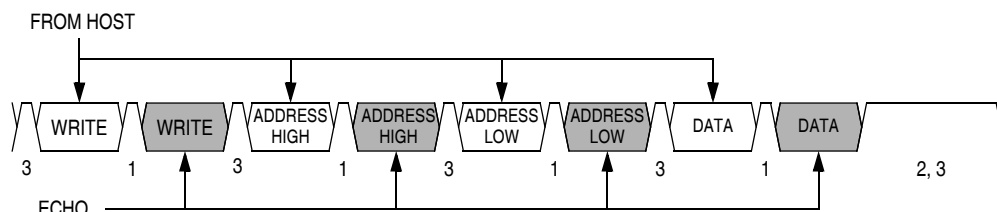
Figure 18-14. Read Transaction
