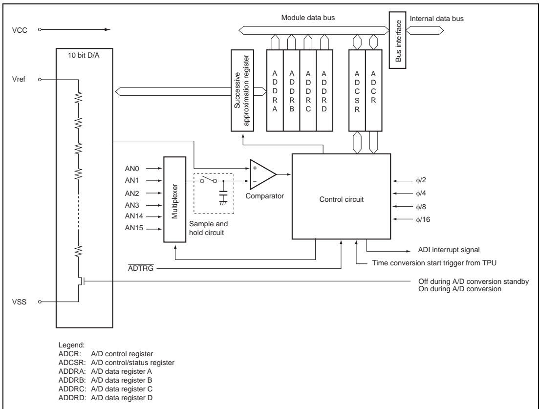
Figure 15.1 Block Diagram of A/D Converter
