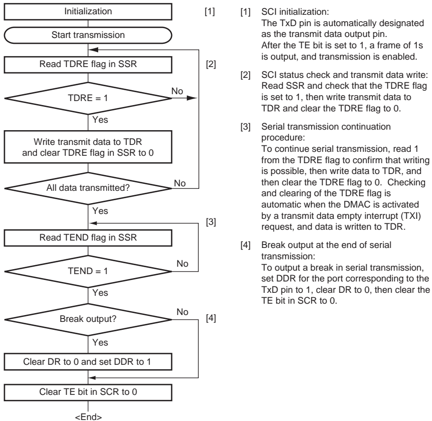
Figure 12.10 Sample Serial Data Transmission Flowchart
