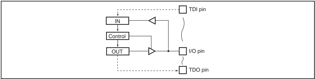
Figure 13.2 Boundary Scan Register Configuration
