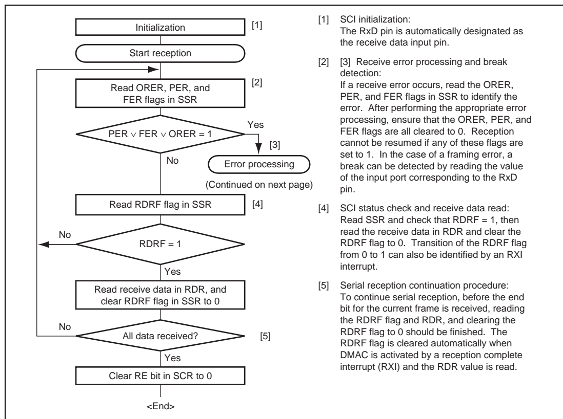
Figure 12.12 Sample Serial Data Reception Flowchart (1)
