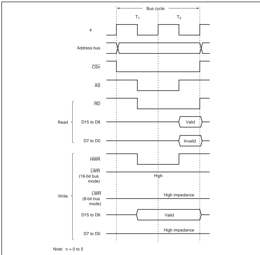
Figure 6.10 Bus Timing for 8-Bit 2-State Access Space
