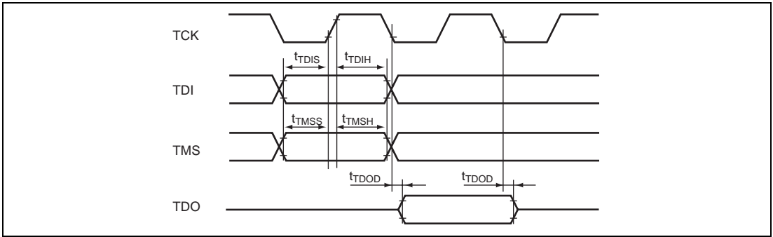
Figure 22.20 Boundary Scan Data Transmission Timing
