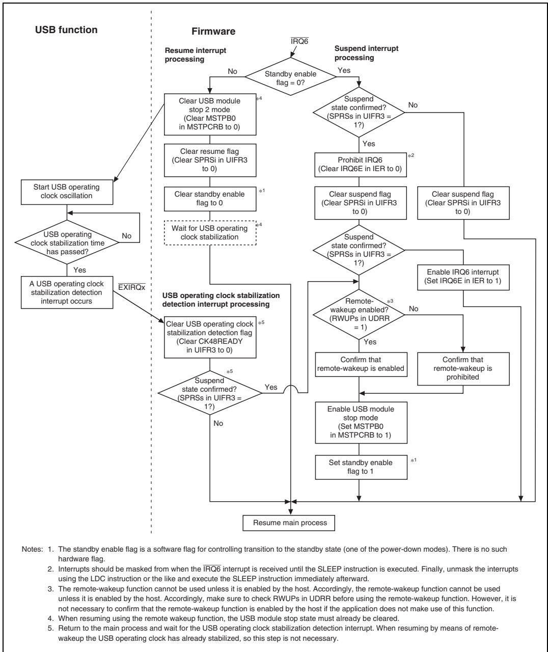
Figure 14.8 Example Flowchart of Suspend and Resume Interrupt Processing
