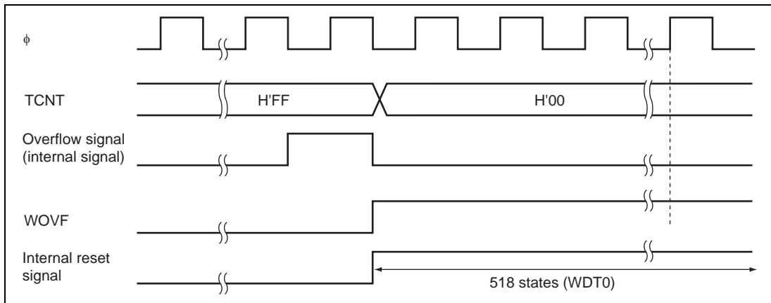
Figure 10.3 Timing of WOVP Setting
