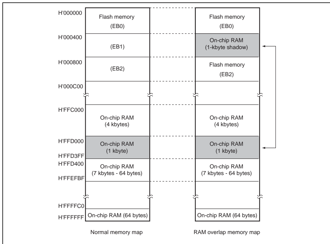
Figure 17.11 Example of RAM Overlap Operation
