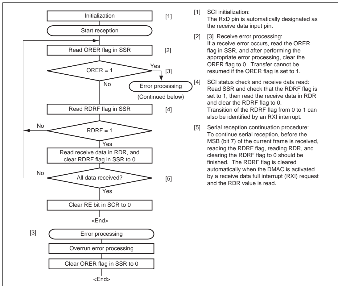
Figure 12.22 Sample Serial Data Reception Flowchart
