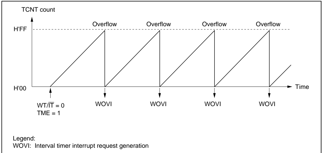
Figure 11.5 Interval Timer Operation
