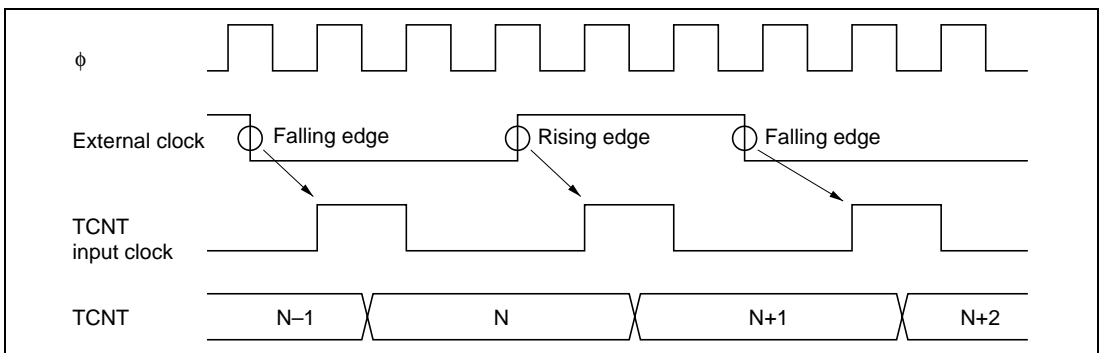
Figure 9.31 Count Timing in External Clock Operation
