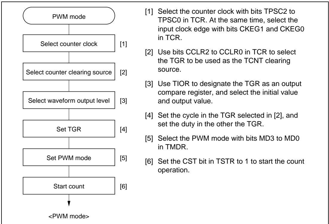
Figure 9.21 Example of PWM Mode Setting Procedure
