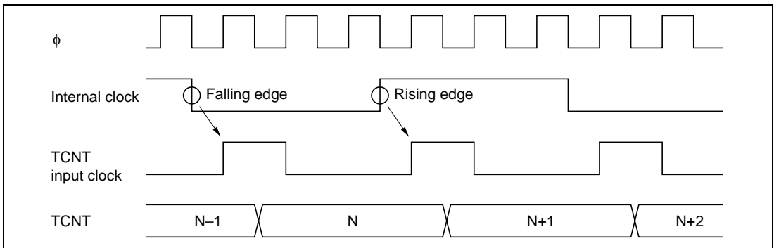
Figure 9.30 Count Timing in Internal Clock Operation
