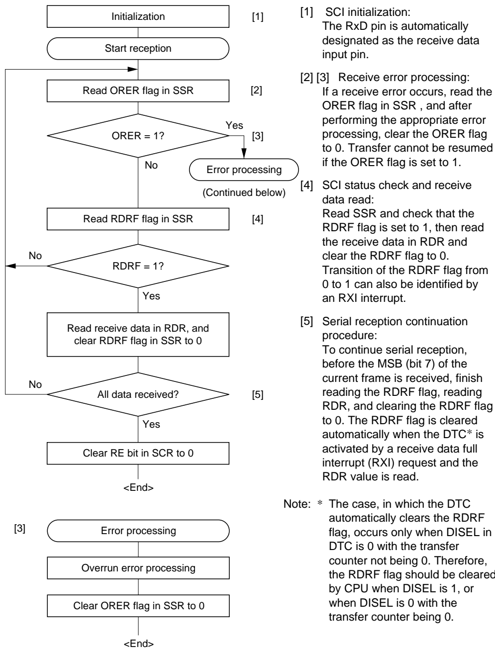
Figure 12.18 Sample Serial Reception Flowchart
