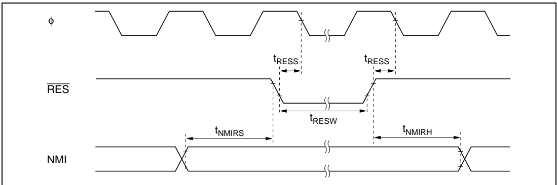
Figure 19.6 Reset Input Timing
