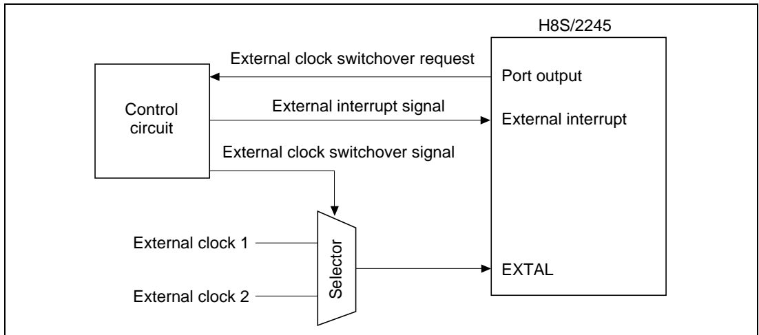
Figure 17.7 Sample External Clock Switching Circuit
