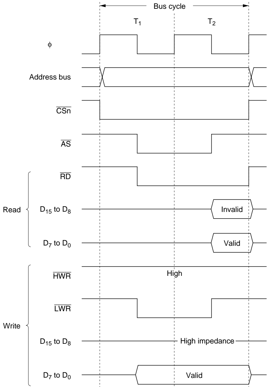
Figure 6.13 Bus Timing for 16-Bit 2-State Access Space (2) (Odd Address Byte Access)
