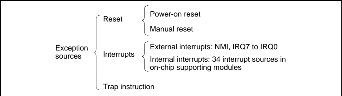
Figure 4.1 Exception Sources
