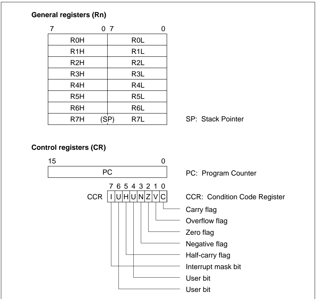
Figure 2-1 CPU Registers
