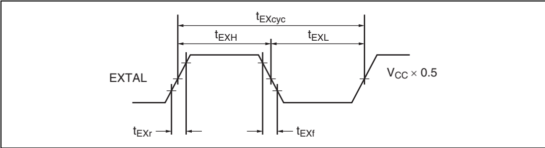
Figure 21.5 External Clock Input Timing
