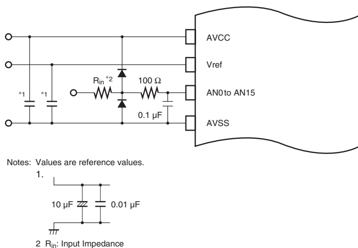
Figure 15.10 Example of Analog Input Protection Circuit
