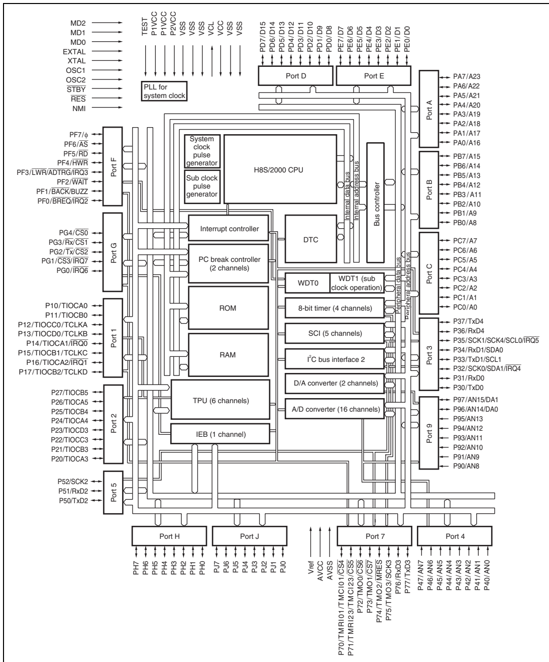
Figure 1.2 Internal Block Diagram of H8S/2552 Group
