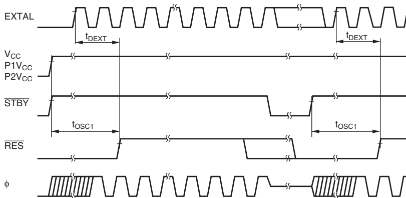
Figure 24.6 Oscillator Settling Timing
