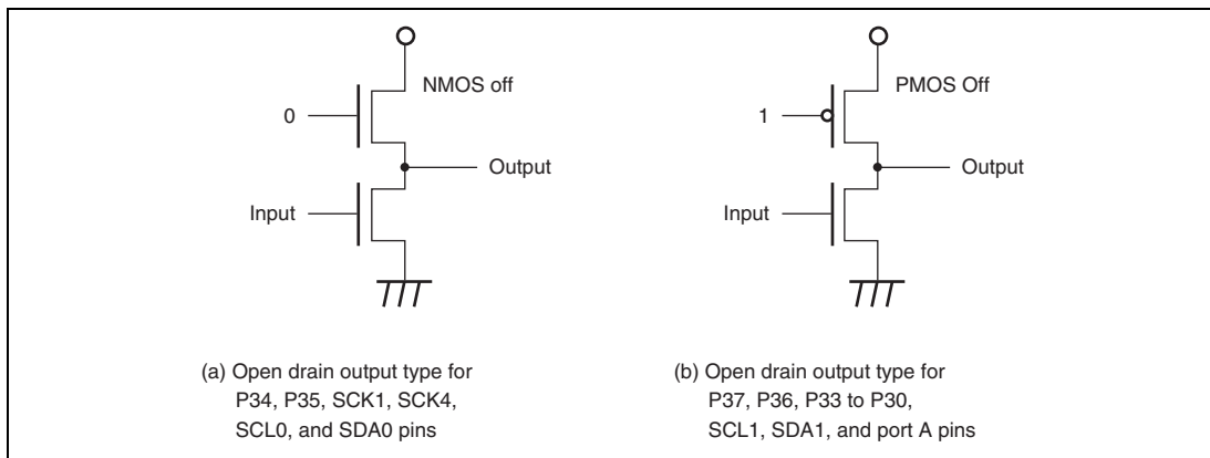
Figure 9.1 Types of Open Drain Outputs
