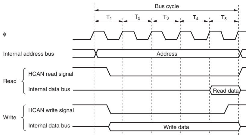
Figure 7.12 On-Chip HCAN Module Access Cycle
