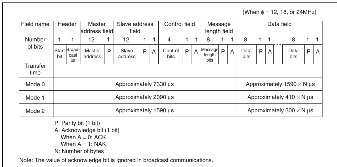
Figure 17.2 Transfer Signal Format
