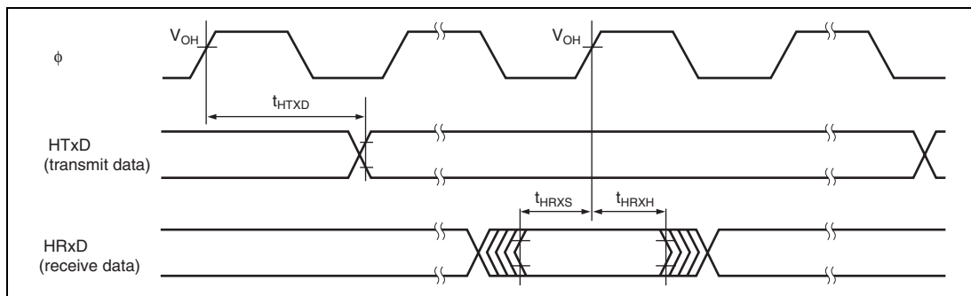
Figure 24.24 HCAN Input/Output Timing
