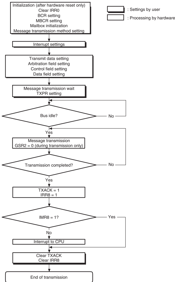
Figure 18.9 Transmission Flowchart
