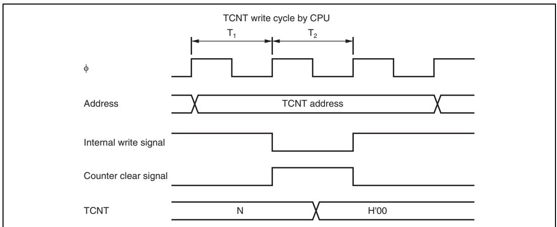
Figure 11.10 Contention between TCNT Write and Clear
