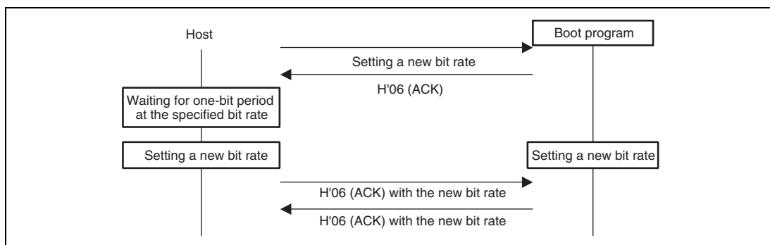
Figure 20.26 New Bit-Rate Selection Sequence
