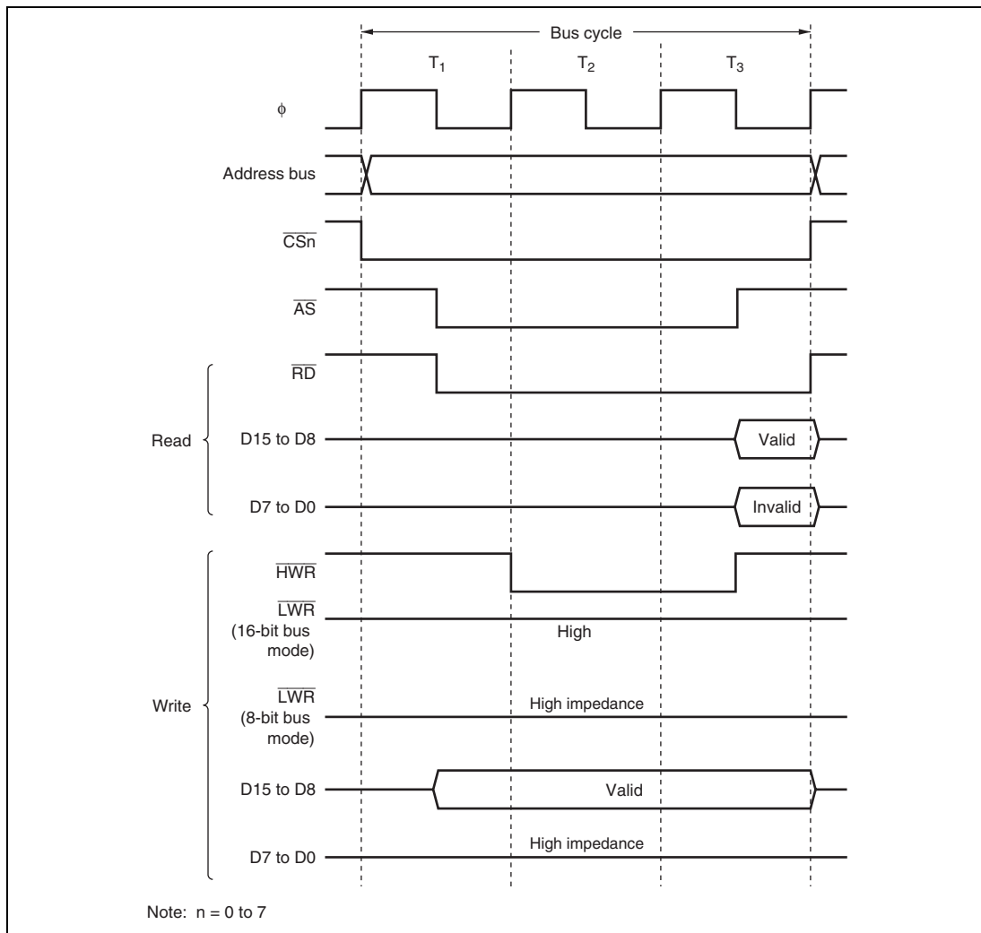
Figure 7.17 Bus Timing for 8-Bit 3-State Access Space
