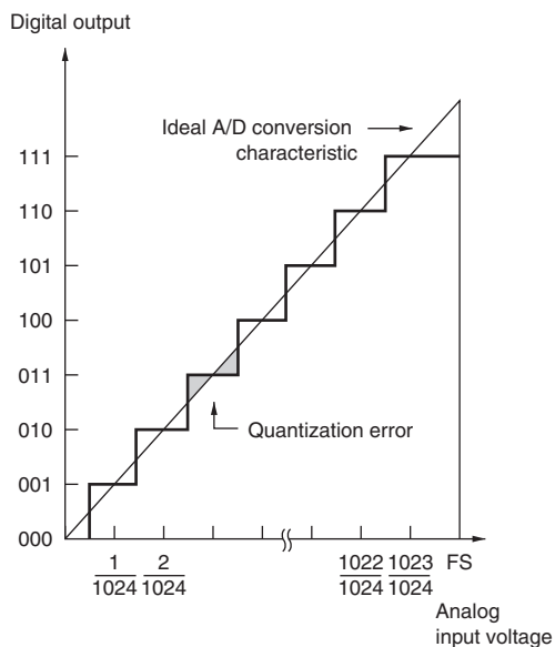
Figure 15.7 A/D Conversion Accuracy Definitions
