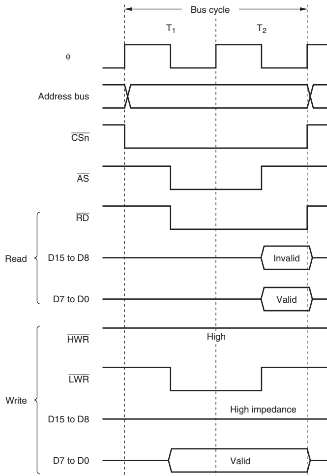
Figure 7.19 Bus Timing for 16-Bit 2-State Access Space (2) (Odd Address Byte Access)
