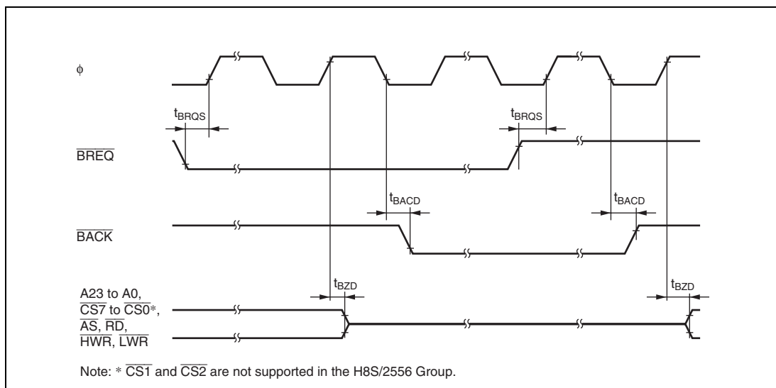
Figure 24.13 External Bus-Released Timing
