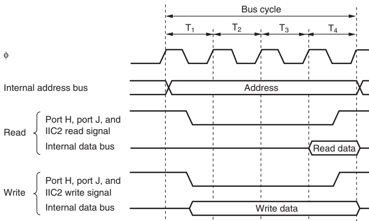
Figure 7.8 On-Chip Port H, Port J, and IIC2 Module Access Cycle
