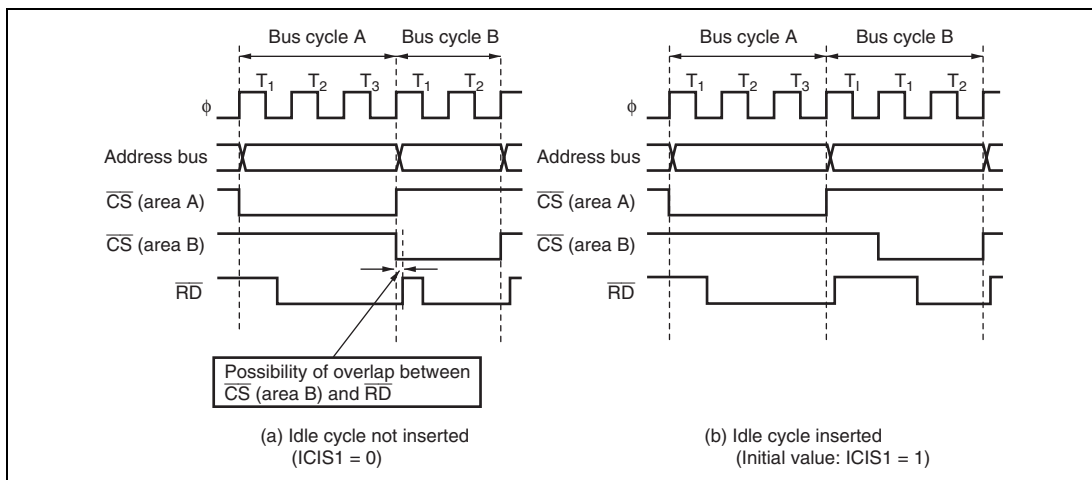
Figure 7.29 Relationship between Chip Select ( \overline{\text{CS}} ) and Read ( \overline{\text{RD}} )
