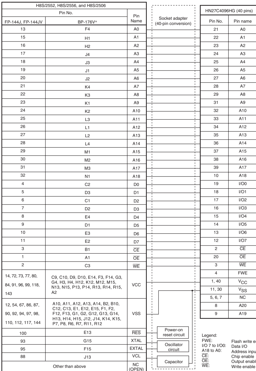
Figure 20.22 Pin arrangement of Socket Adapter
