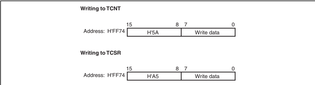
Figure 12.6 Writing to TCNT and TCSR (WDT_0)
