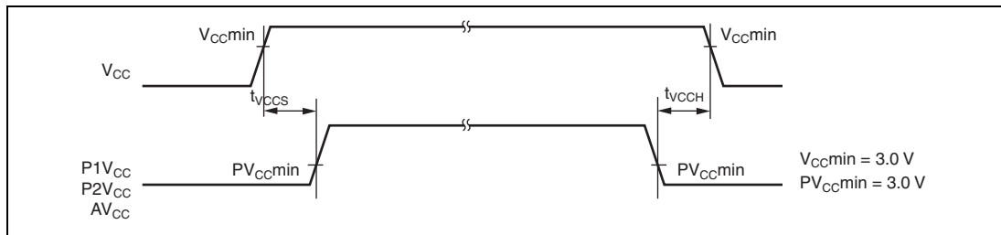
Figure 24.3 Power-On/Off Timing
