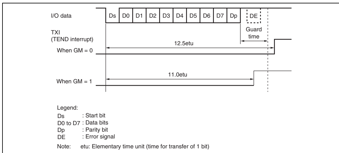
Figure 13.27 TEND Flag Generation Timing in Transmission Operation
