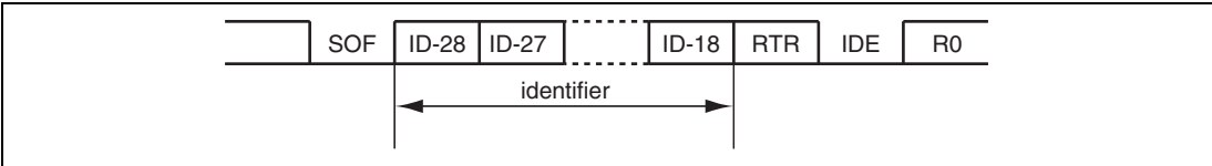
Figure 18.3 Standard Format
