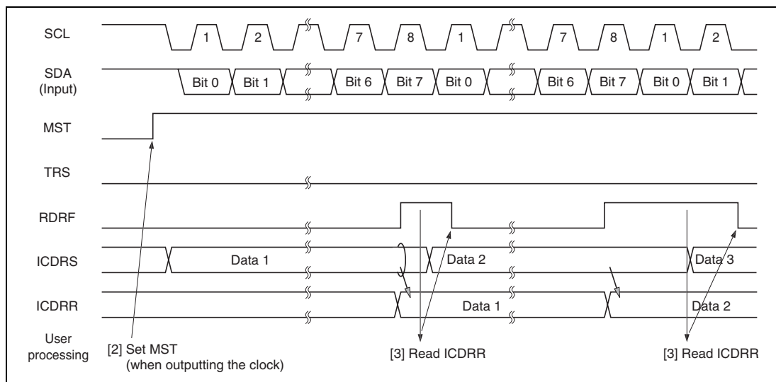
Figure 14.15 Receive Mode Operation Timing
