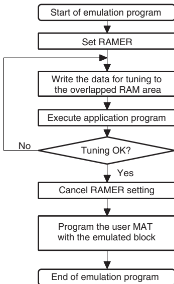
Figure 20.17 Emulation of Flash Memory in RAM
