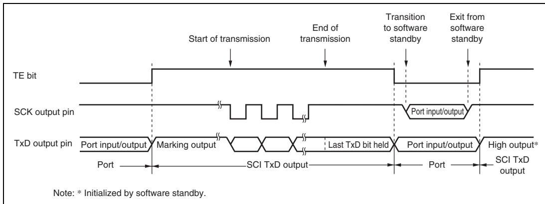
Figure 13.36 Clocked Synchronous Transmission Using Internal Clock
