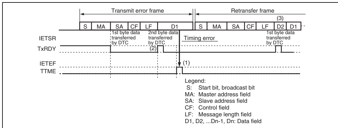
Figure 17.15 Error Processing in Transfer
