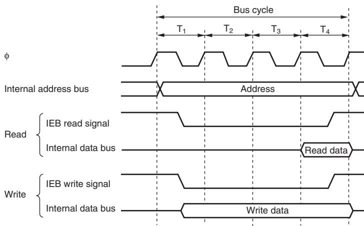
Figure 7.10 On-Chip IEB Module Access Cycle
