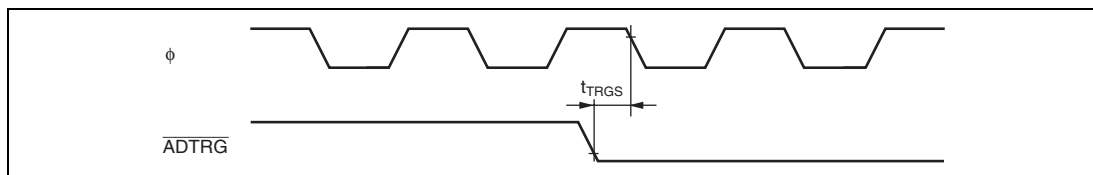
Figure 24.23 External Trigger Input Timing for A/D Converter
