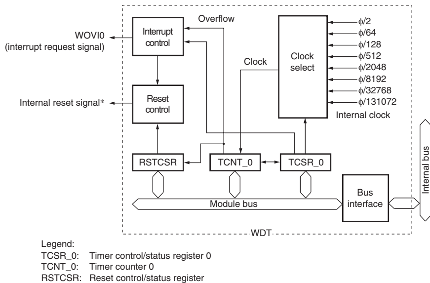
Figure 12.1 Block Diagram of WDT_0 (1)
