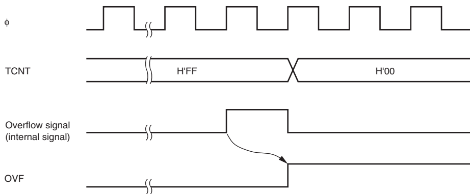
Figure 12.4 Timing of OVF Setting
