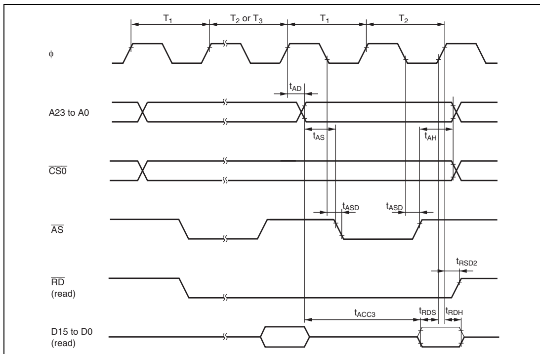
Figure 24.12 Burst ROM Access Timing: Two-State Access
