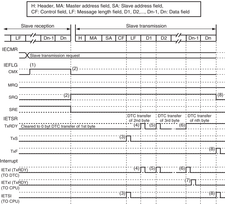
Figure 17.12 Slave Transmit Operation Timing
