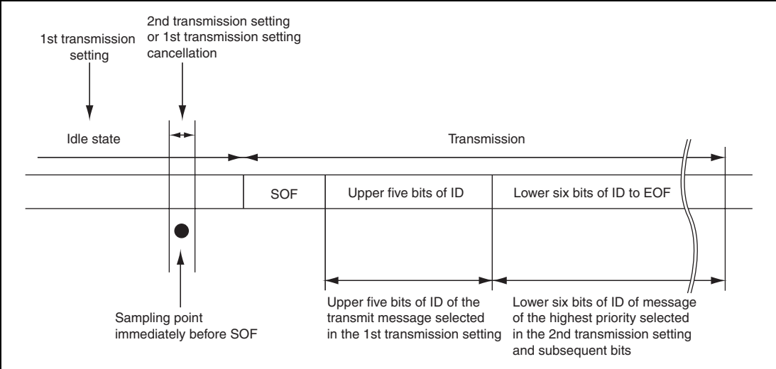
Figure 18.17 HCAN Transmit Procedure
