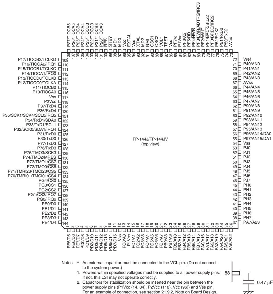
Figure 1.6 Pin Arrangement of H8S/2506 Group (FP-144J and FP-144JV)
