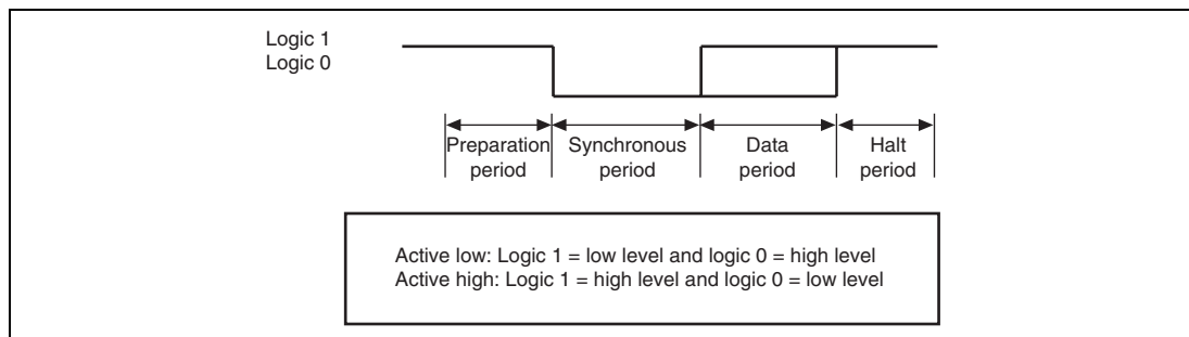
Figure 17.5 IEBus Bit Format (Conceptual Diagram)
