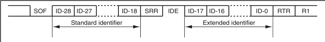
Figure 18.4 Extended Format
