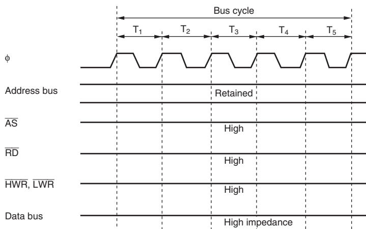
Figure 7.13 Pin States during On-Chip HCAN Module Access
