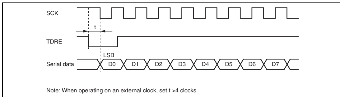
Figure 13.33 Example of Clocked Synchronous Transmission by DTC
