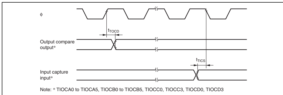
Figure 24.15 TPU Input/Output Timing
