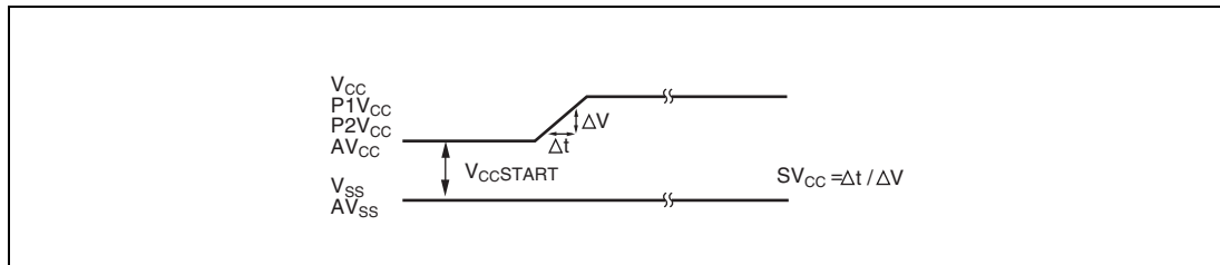
Figure 24.4 Power-On Timing
