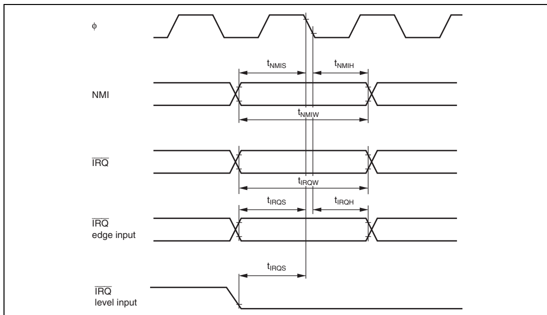
Figure 24.8 Interrupt Input Timing
