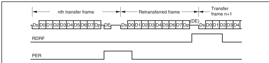
Figure 13.29 Retransfer Operation in SCI Receive Mode
