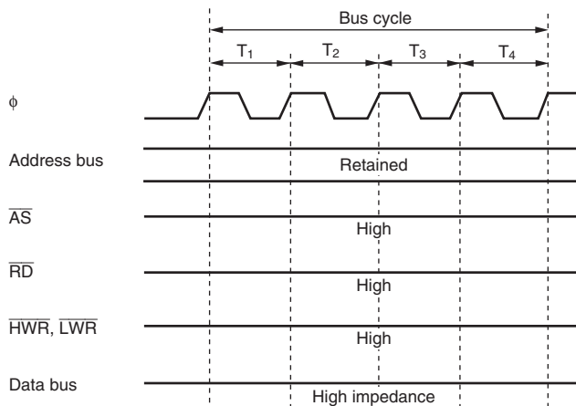
Figure 7.11 Pin States during On-Chip IEB Module Access
