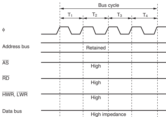
Figure 7.9 Pin States during On-Chip Port H, Port J, and IIC2 Module Access
