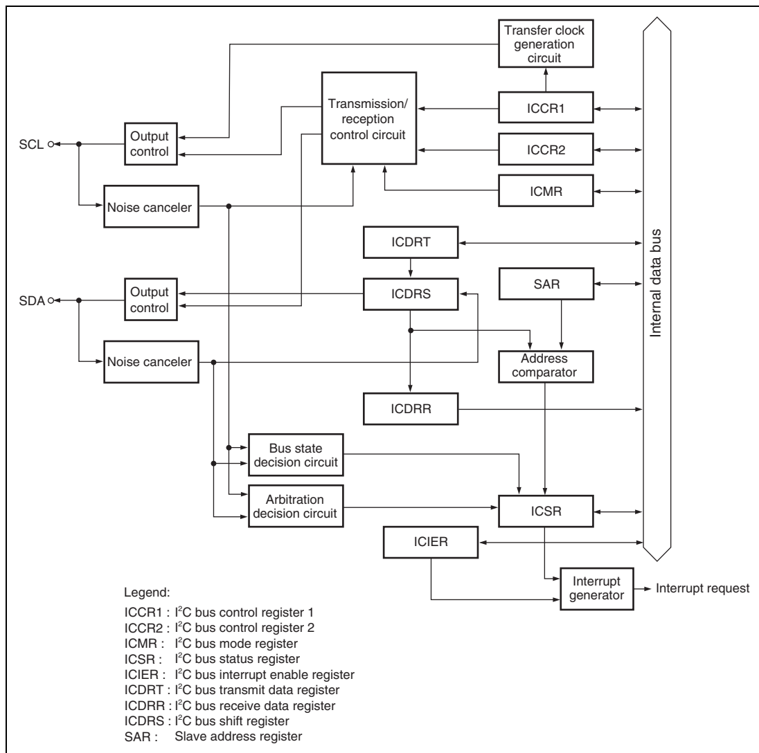
Figure 14.1 Block Diagram of I 2 C Bus Interface 2
