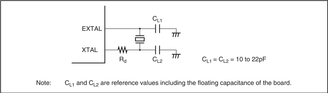
Figure 21.2 Connection of Crystal Resonator (Example)
