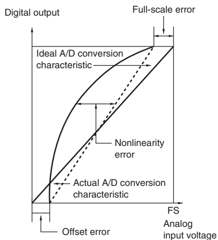
Figure 15.8 A/D Conversion Accuracy Definitions
