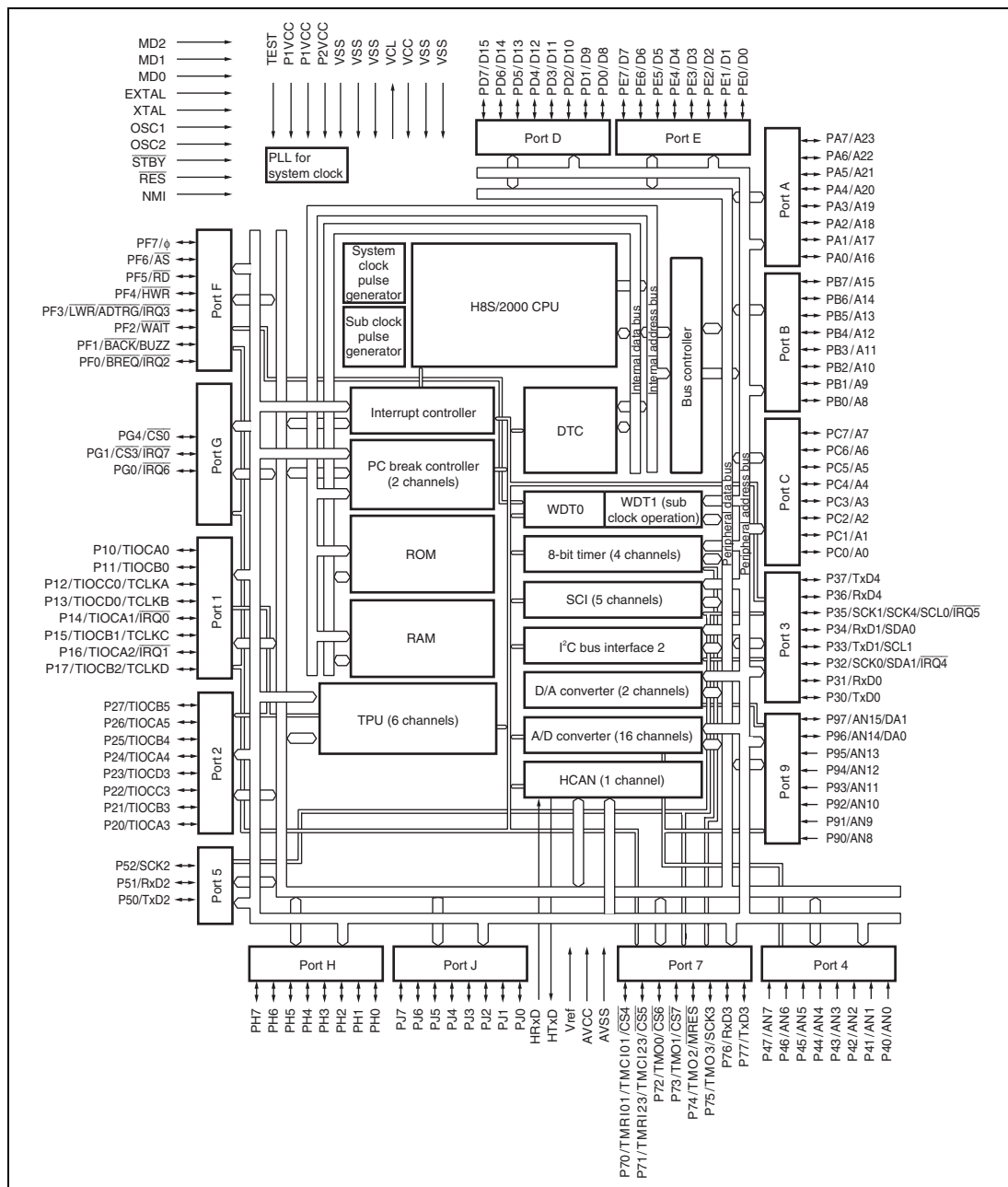
Figure 1.1 Internal Block Diagram of H8S/2556 Group
