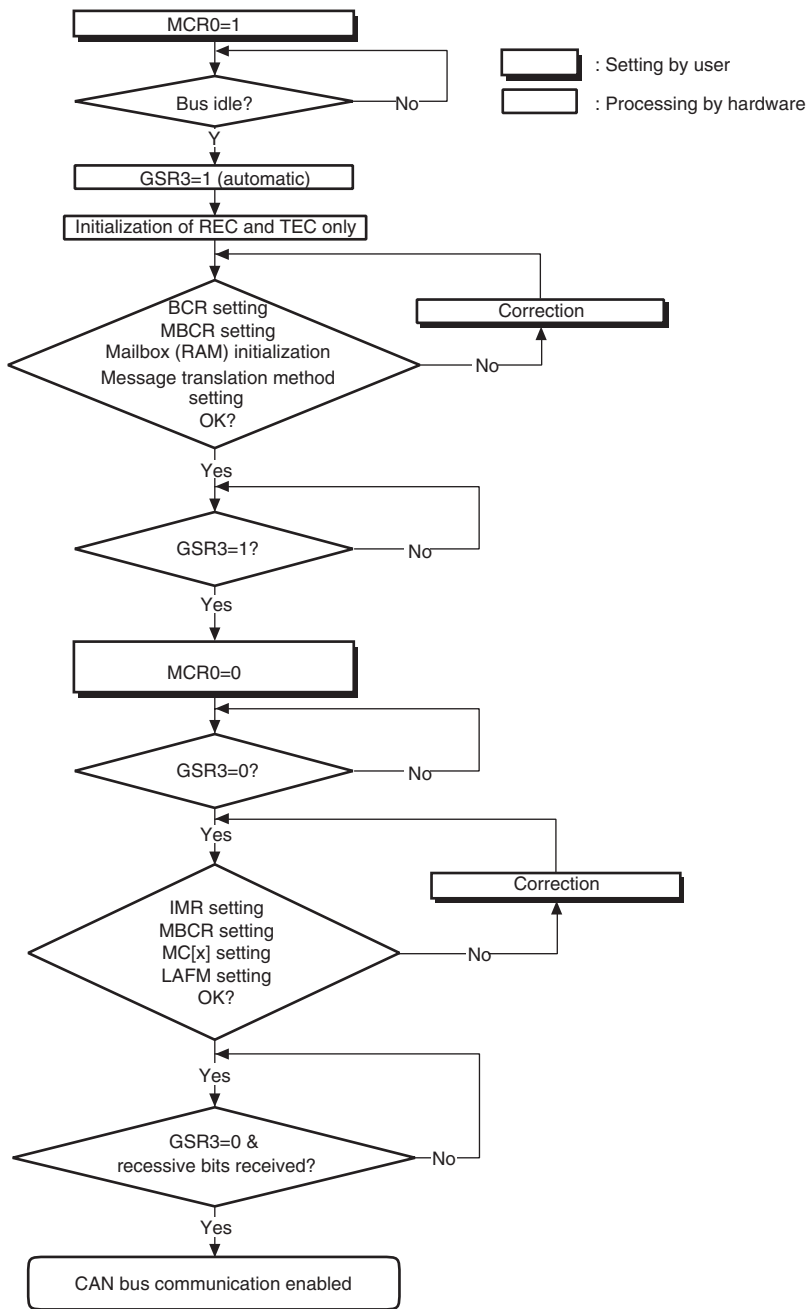
Figure 18.7 Software Reset Flowchart
