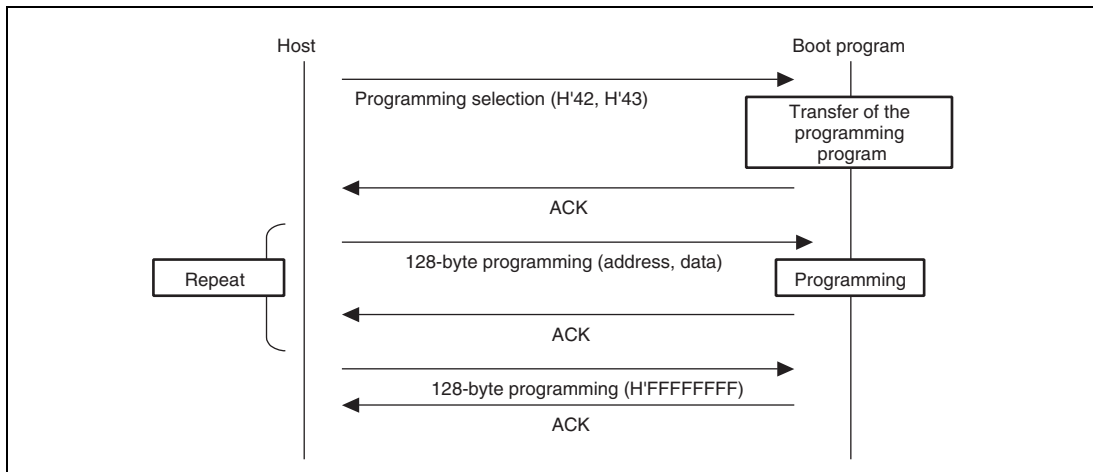
Figure 20.27 Programming Sequence
