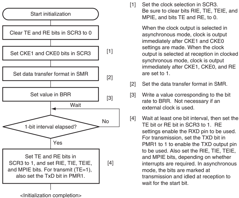
Figure 17.4 Sample SCI3 Initialization Flowchart
