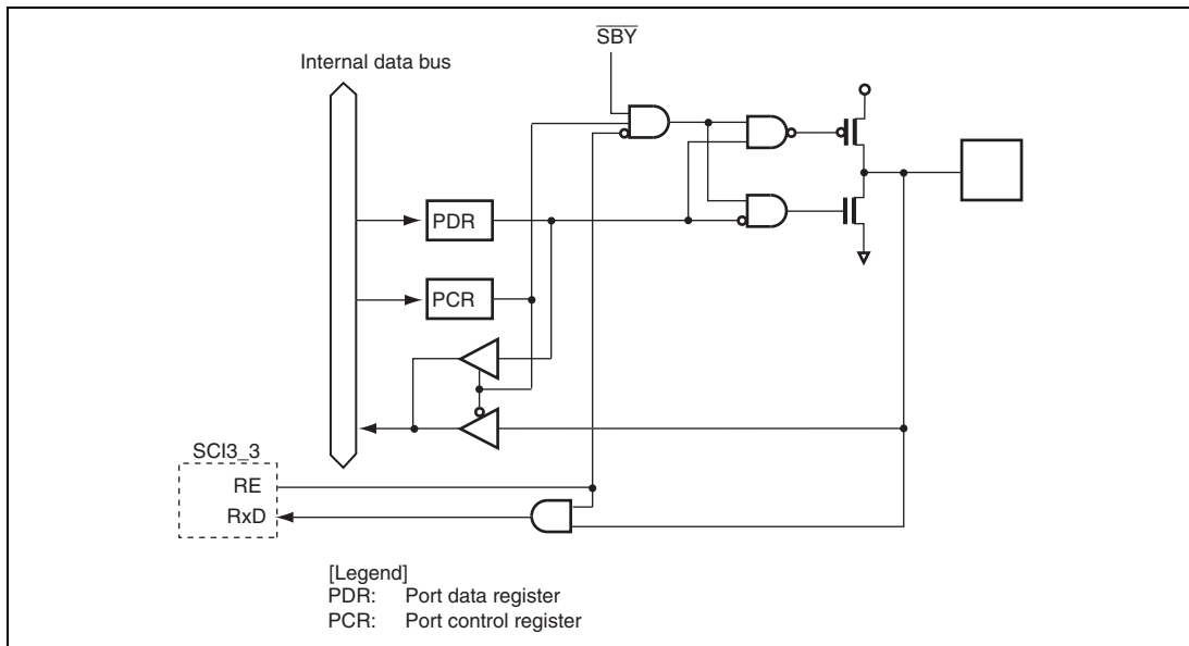
Figure B.28 Port 9 Block Diagram (P91)
