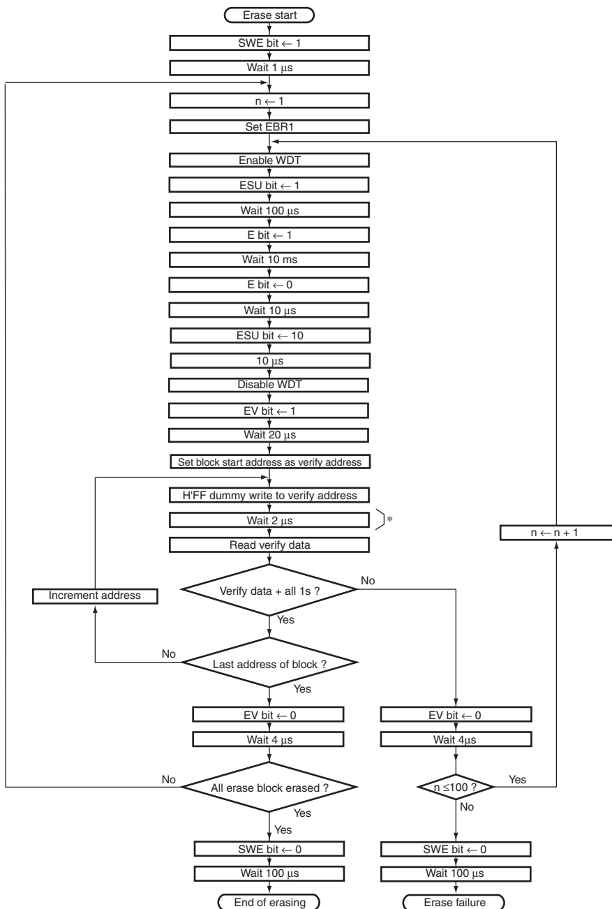
Figure 7.4 Erase/Erase-Verify Flowchart
