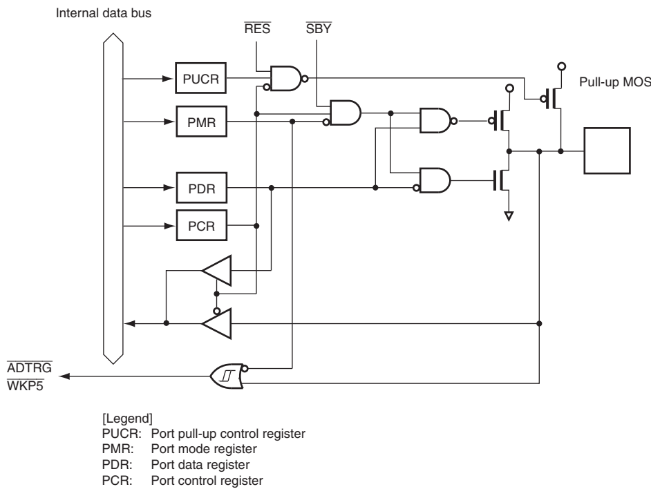
Figure B.13 Port 5 Block Diagram (P55)
