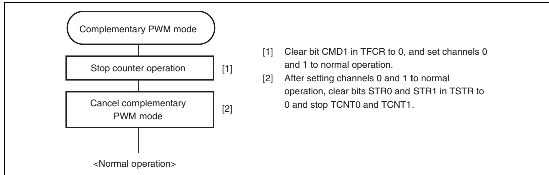
Figure 14.30 Canceling Procedure of Complementary PWM Mode
