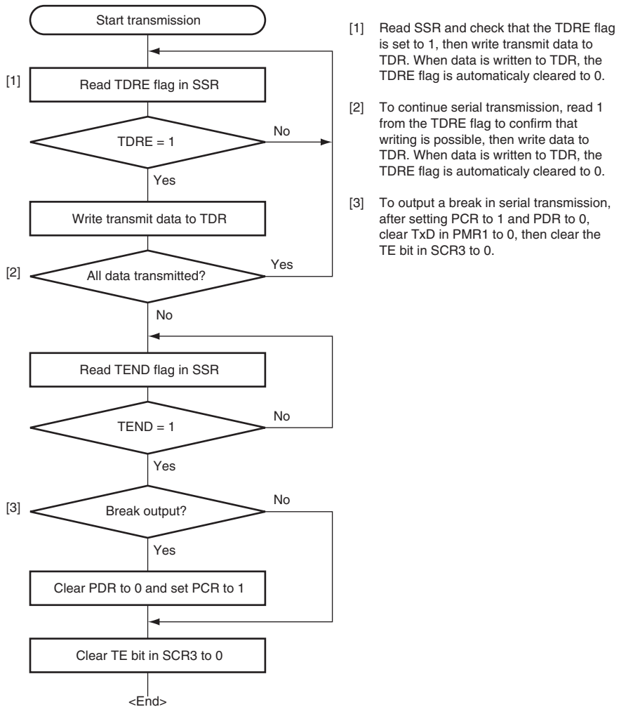
Figure 17.6 Sample Serial Transmission Data Flowchart (Asynchronous Mode)
