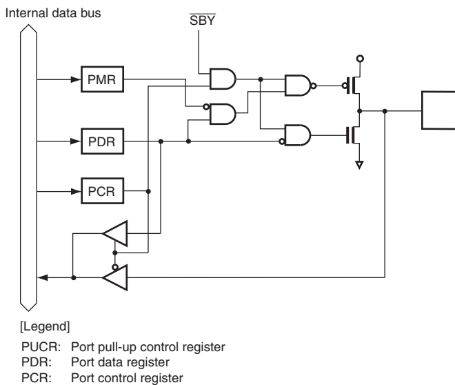
Figure B.7 Port 2 Block Diagram (P24, P23)
