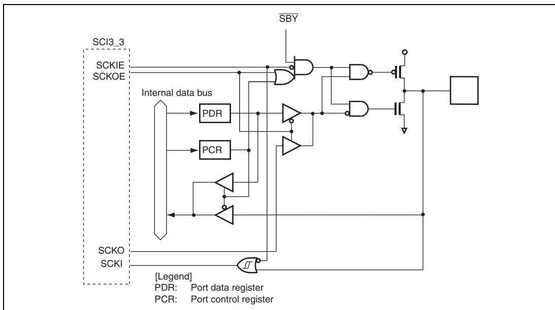
Figure B.29 Port 9 Block Diagram (P90)
