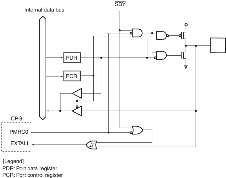
Figure B.26 Port B Block Diagram (PC0)
