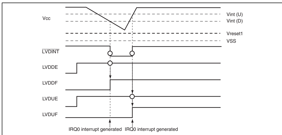
Figure 19.5 Operational Timing of LVDI Circuit
