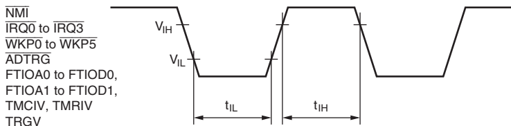
Figure 22.3 Input Timing
