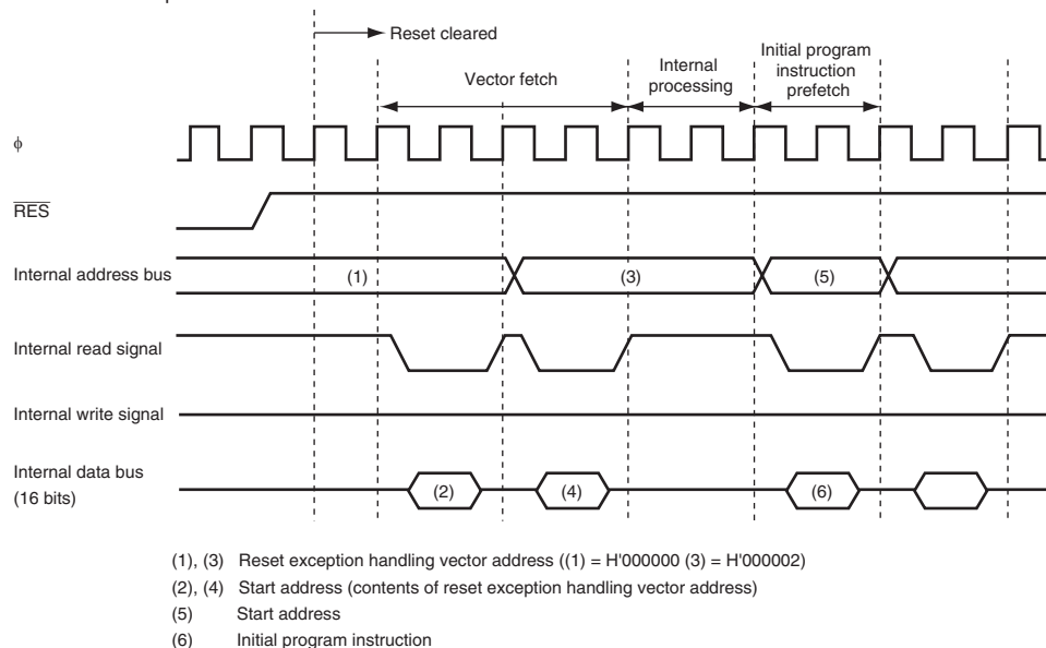
Figure 3.1 Reset Sequence
