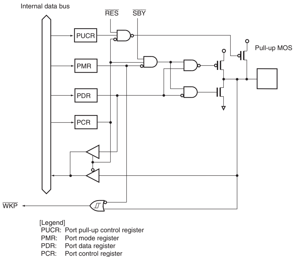
Figure B.14 Port 5 Block Diagram (P54 to P50)
