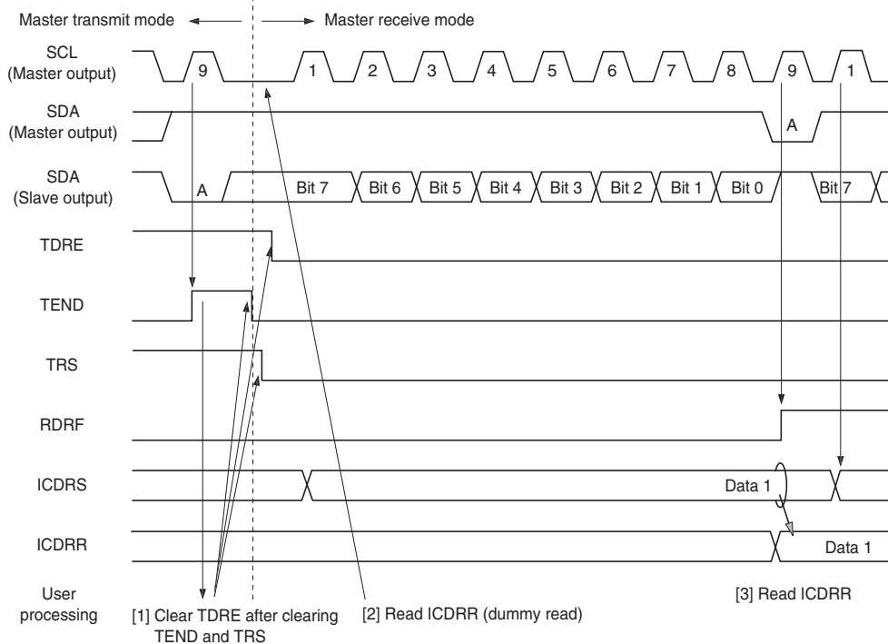
Figure 17.7 Master Receive Mode Operation Timing (1)
