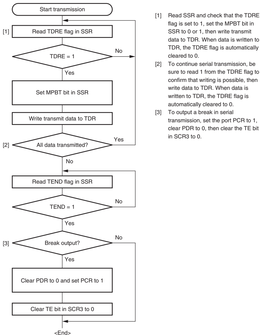
Figure 16.16 Sample Multiprocessor Serial Transmission Flowchart
