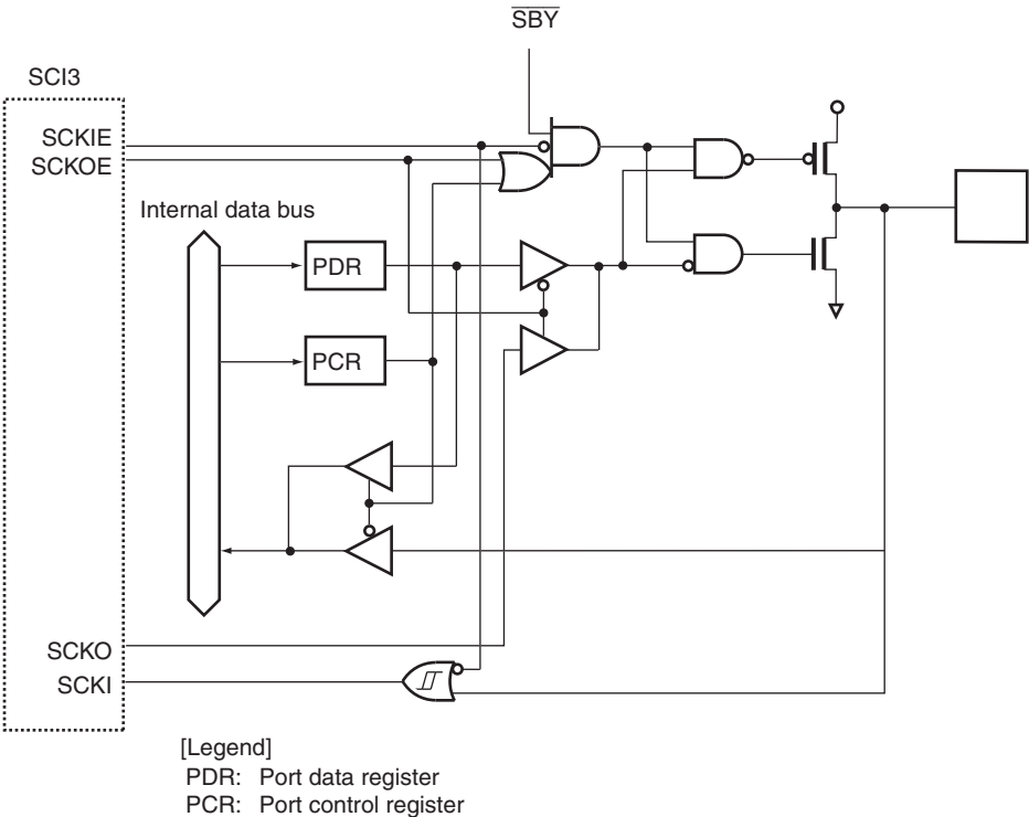
Figure B.10 Port 2 Block Diagram (P20)
