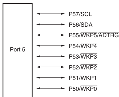
Figure 9.4 Port 5 Pin Configuration
