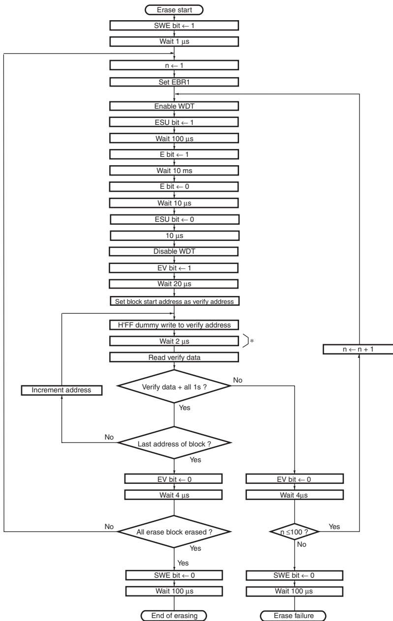
Figure 7.4 Erase/Erase-Verify Flowchart
