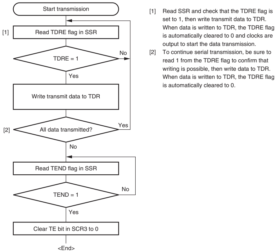
Figure 16.11 Sample Serial Transmission Flowchart (Clocked Synchronous Mode)
