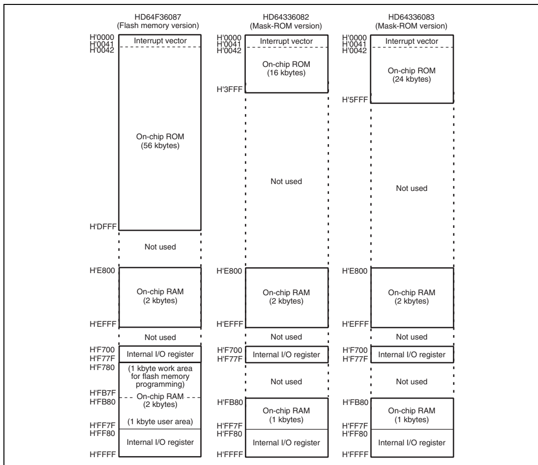
Figure 2.1 Memory Map (1)
