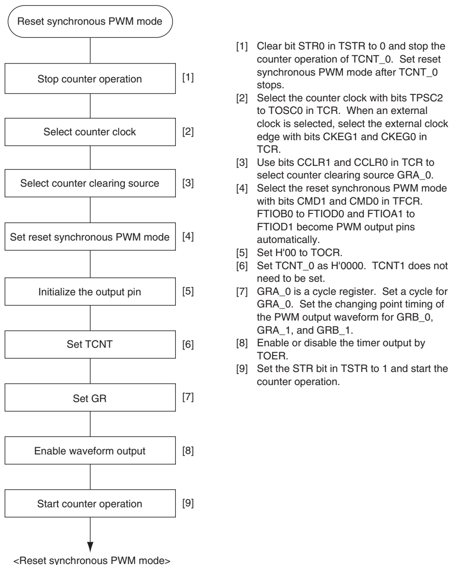
Figure 13.26 Example of Reset Synchronous PWM Mode Setting Procedure
