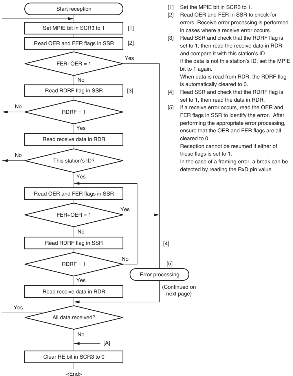
Figure 16.17 Sample Multiprocessor Serial Reception Flowchart (1)
