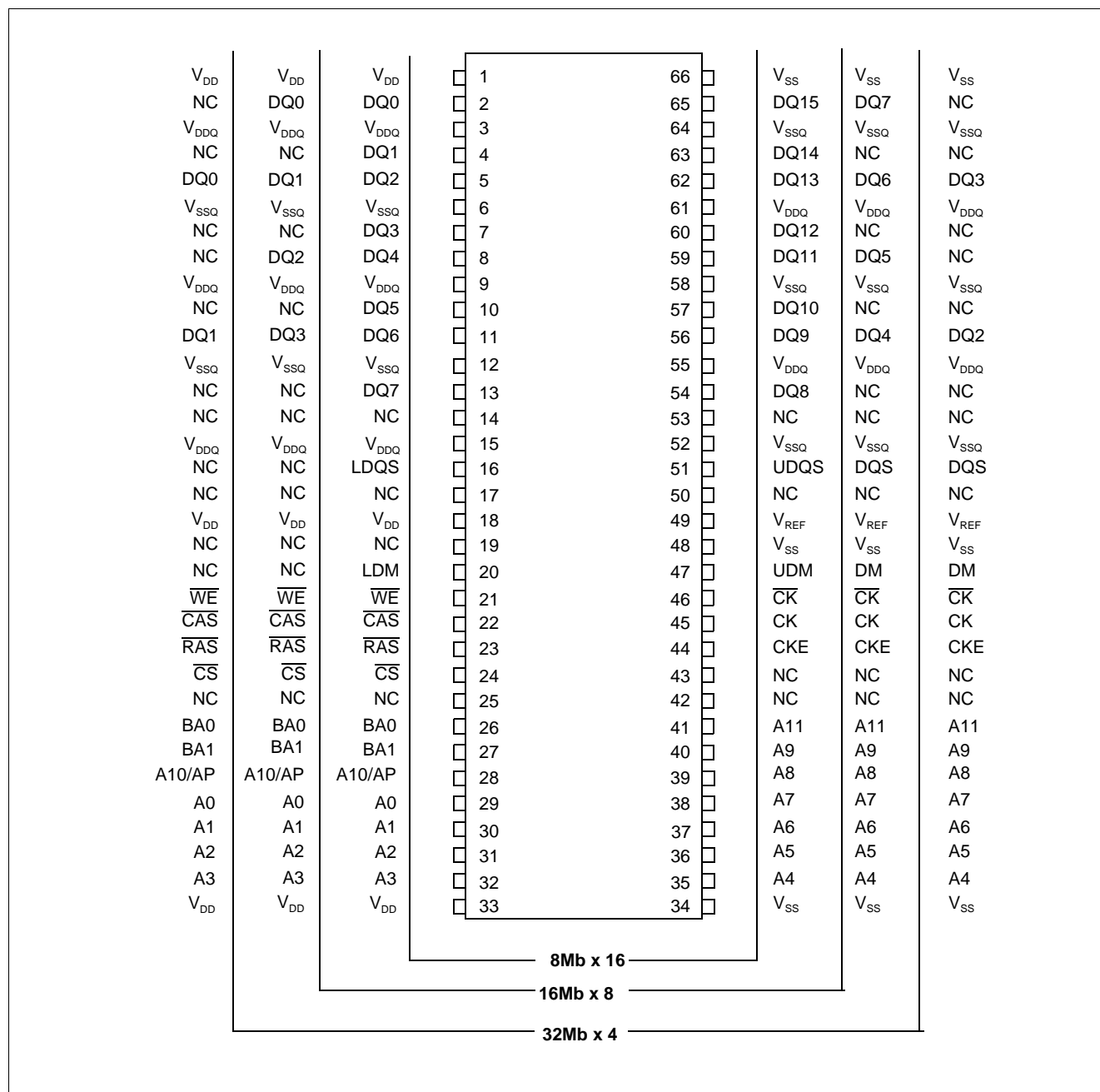
Figure 1 Pin Configuration
