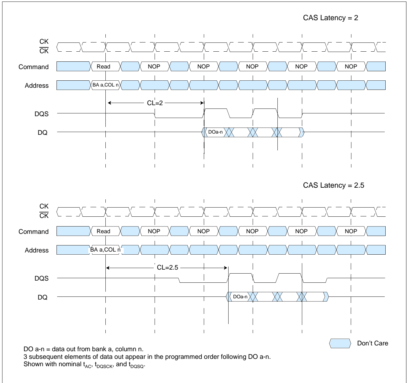
Figure 9 Read Burst: CAS Latencies (Burst Length = 4)
