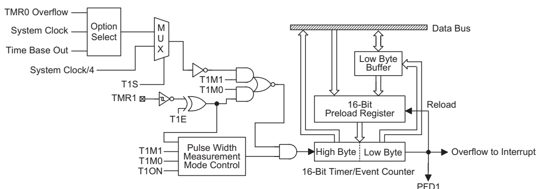
Timer/Event Counter 1
