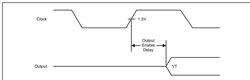
Figure 8-6. Output Enable Delay
