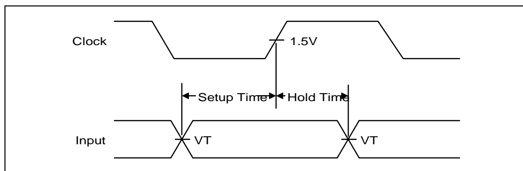
Figure 8-4. Float Delay
