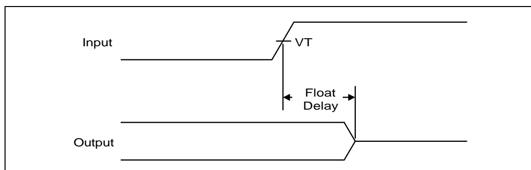
Figure 8-5. Pulse Width
