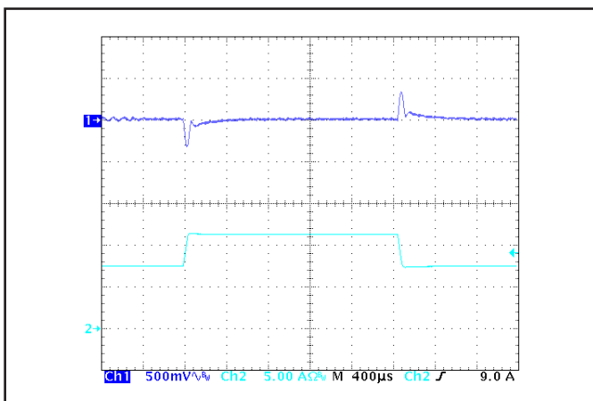
Figure 5: Output voltage response to step-change in load current (50%-75%-50% of I out (max); dI/dt = 0.1 A/μs). Load cap: 1 μF ceramic and 15 μF tantalum capacitors. Ch 1: Vout (500 mV/div), Ch 2: Iout (5 A/div).
