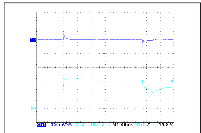
Figure 6: Output voltage response to step-change in input voltage (500 V/ms). Load cap: 100 μF, electrolytic output capacitance. Ch 1: Vout (500 mV/div), Ch 2: Vin (10 V/div).
