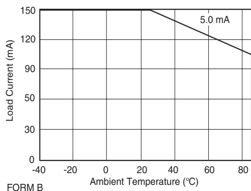
Figure 2. Recommended Operating Conditions
