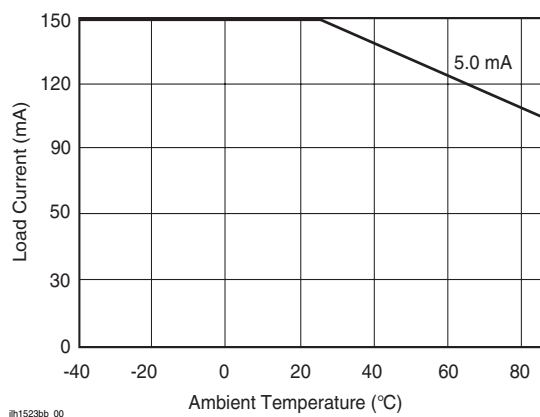
Figure 1. Recommended Operating Conditions
