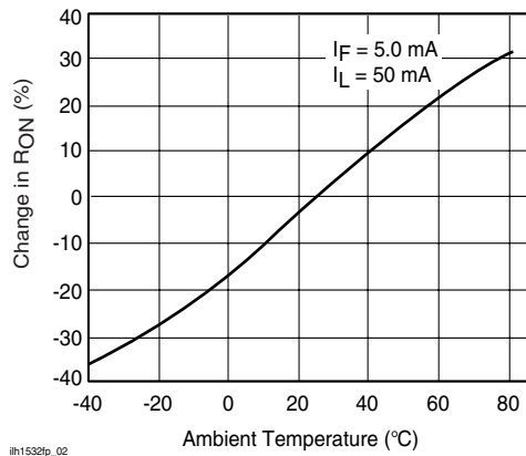
Figure 2. ON-Resistance vs. Temperature
