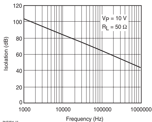
Figure 14. Output Isolation
