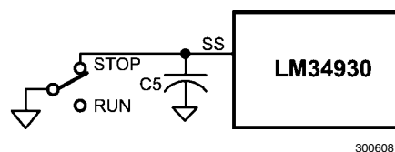
FIGURE 3. Shutdown Implementation
