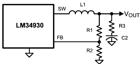
FIGURE 8. Basic Ripple Configuration
