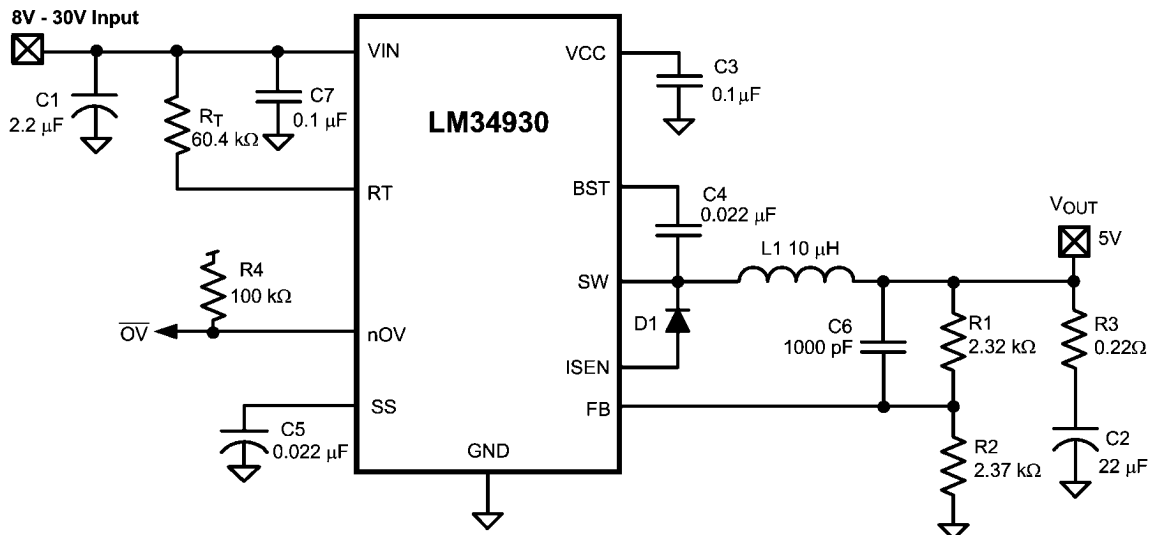
FIGURE 4. Example Circuit
