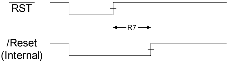
Figure 18-9. External Reset Timing ( \overline{\text{RST}} )
