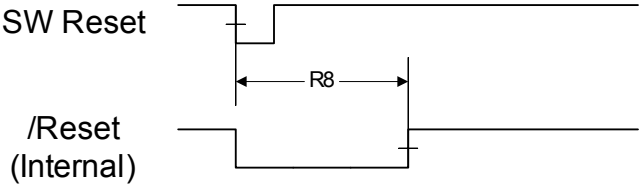
Figure 18-12. Software Reset Timing
