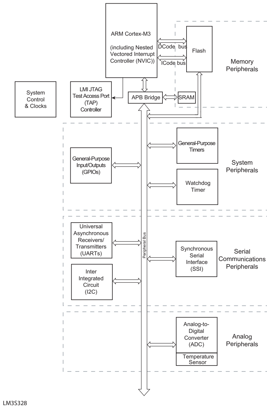
Figure 1-1. Stellaris® High-Level Block Diagram
