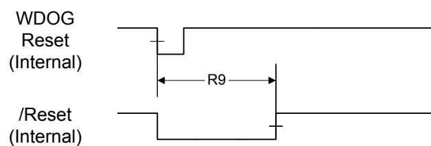
Figure 19-13. Watchdog Reset Timing
