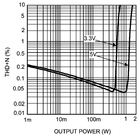
THD+N vs Output Power V_{DD} = 3.3V & 5V , R_L = 8\Omega BTL, f = 1kHz Mode 2, 80kHz BW
