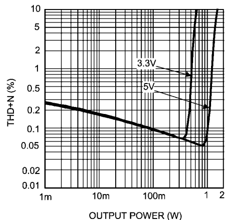
THD+N vs Output Power V_{DD} = 3.3V & 5V , R_L = 8\Omega , f = 1kHz Mode 5, 80kHz BW
