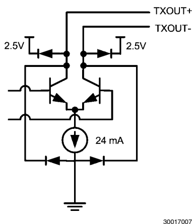
FIGURE 5. Simplified SDI Output Circuit
