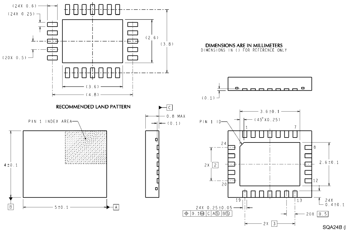
24-Pin LLP Order Number LMH0346SQ NS Package Number SQA24B
