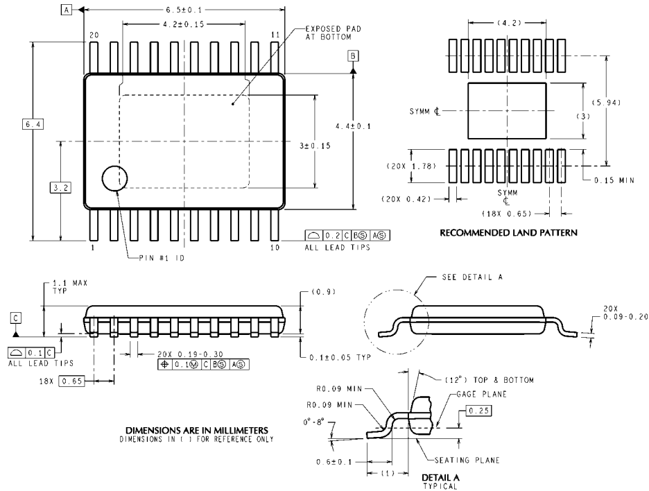
20-Pin e-TSSOP Order Number LMH0346MH NS Package Number MXA20A
