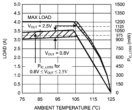
Current Derating V_{IN} = 3.3V , \theta_{JA} = 20^\circ\text{C/W}
