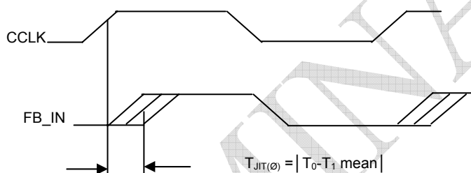
Figure 13. I/O Jitter
