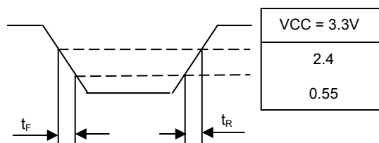
Figure 16. Output Transition Time Test Reference
