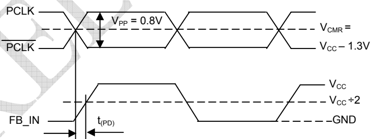
Figure 11. Propagation Delay ( t_{PD} ). Static phase offset test reference
