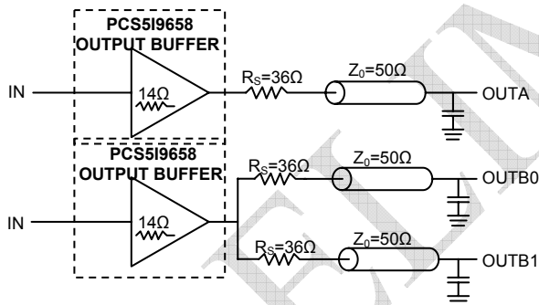
Figure 6. Single versus Dual Transmission Lines
