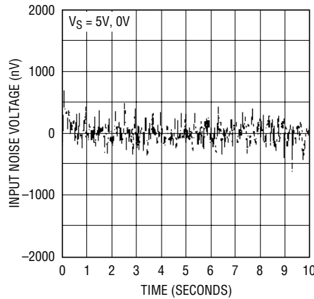
0.1Hz to 10Hz Input Voltage Noise
