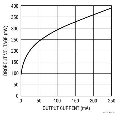
Dropout Voltage
