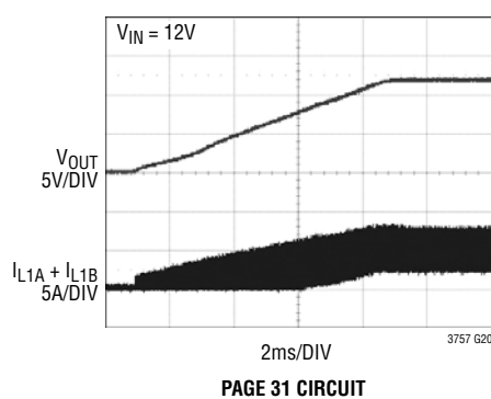
Typical Start-Up Waveforms
