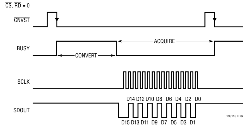
Conversion Timing Using the Serial Interface
