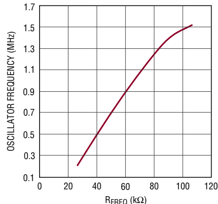
Oscillator Frequency vs R_{FREQ}
