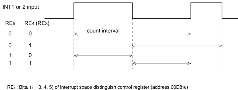
Fig. 36 Interrupt space distinguish control register setting value and the measuring interval
