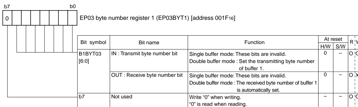
Fig. 3.4.37 Structure of EP03 byte number register 1
