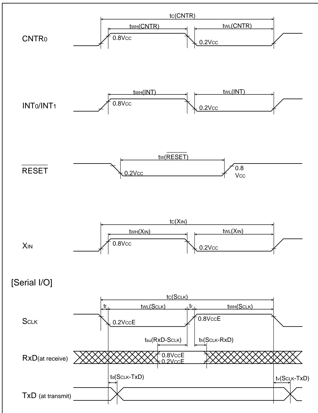
Fig. 3.1.4 Timing chart (1)
