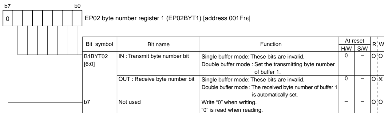
Fig. 3.4.36 Structure of EP02 byte number register 1
