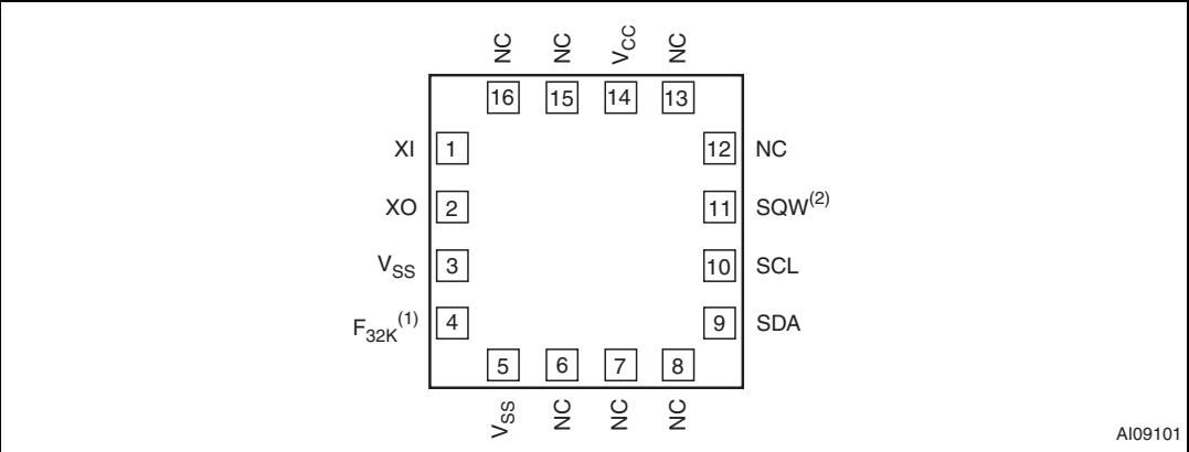
Figure 7. M41T64 connections
