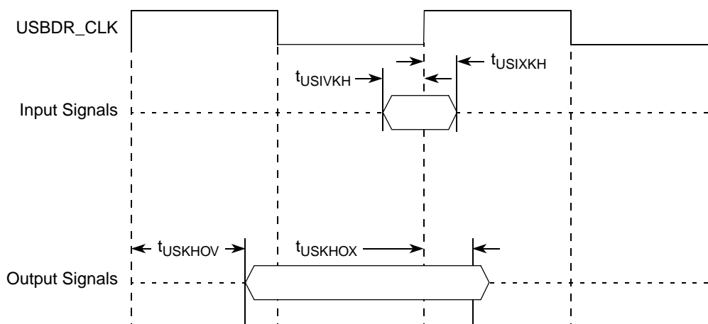
Figure 14. USB Signals
