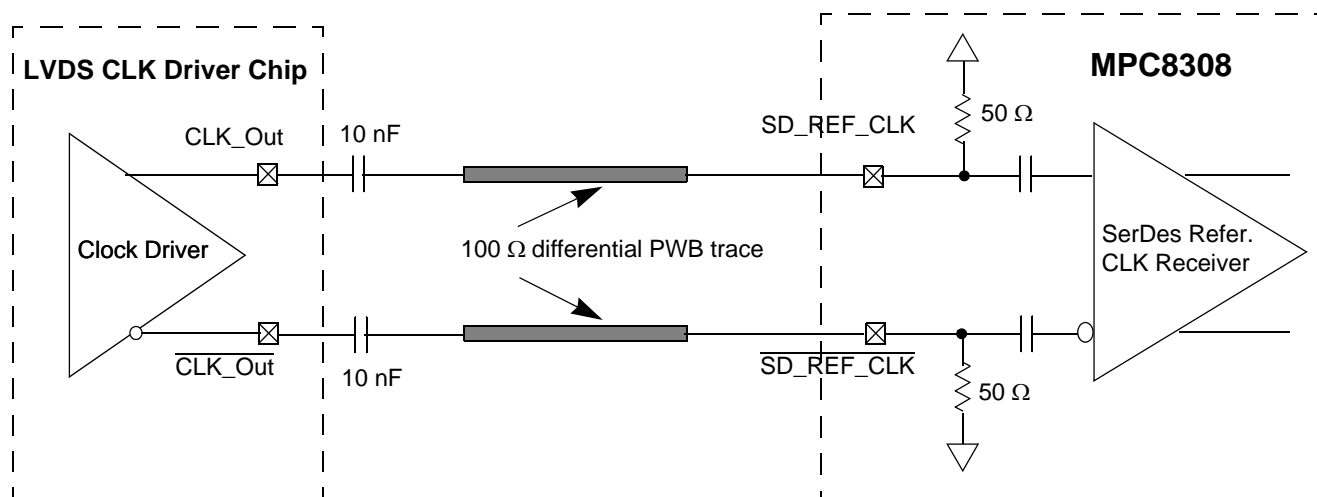
Figure 21. AC-Coupled Differential Connection with LVDS Clock Driver (Reference Only)
