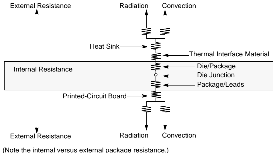
Figure 58. Package with Heat Sink Mounted to a Printed-Circuit Board
