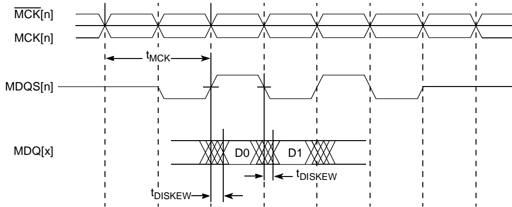
Figure 3. DDR SDRAM Input Timing Diagram ( t_{\text{DISKEW}} )
