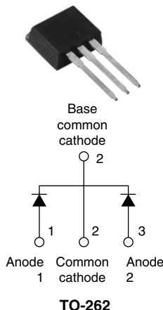
MURB1020CT-1PbF
