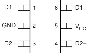
TPD4S009...DBV OR DCK PACKAGE (TOP VIEW)
