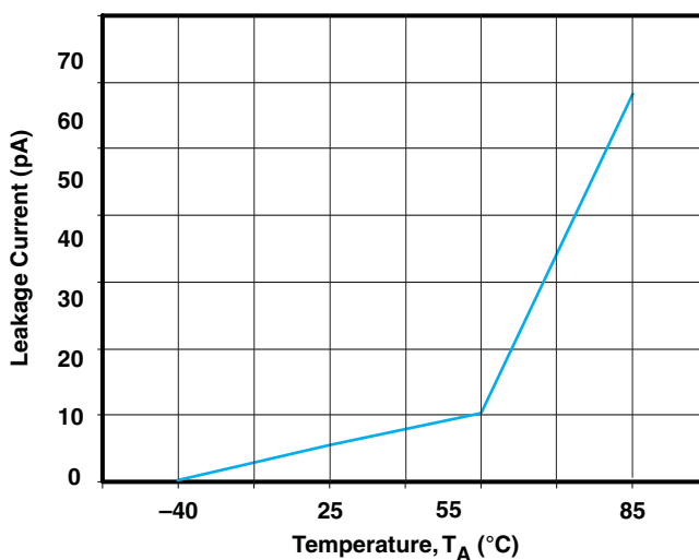
Figure 2. Leakage Current vs Temperature ( V_{IO} = 2.5 V)
