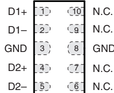
TPD4S010...DQA PACKAGE (TOP VIEW)
