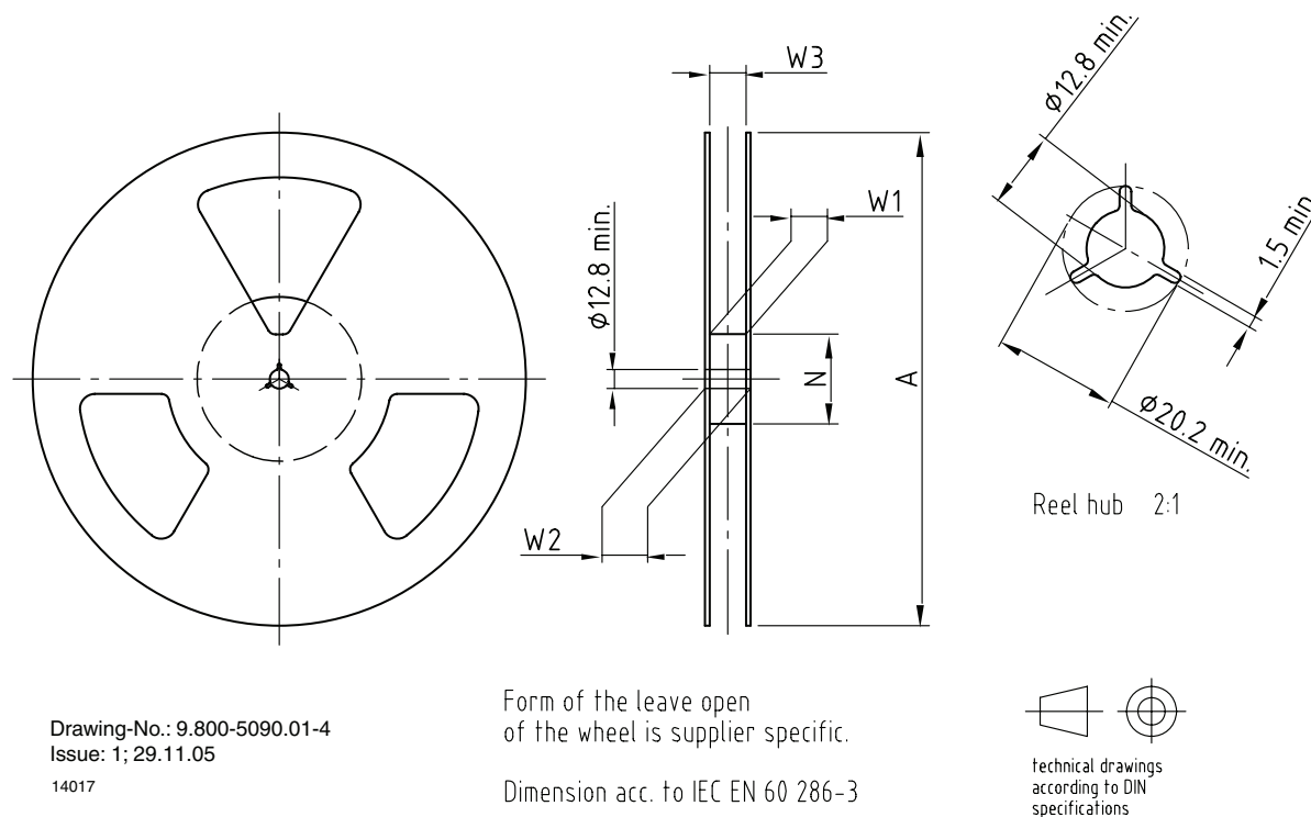
Figure 9. Reel Drawing
