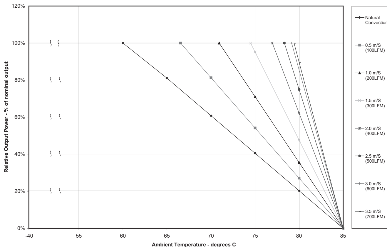
FIGURE 1. OUTPUT DERATING
