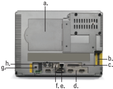
Figure 2. TPC-2512 Connectivity
