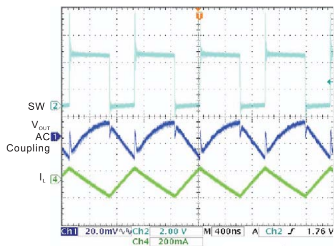
Switching Waveform
