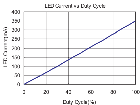
Figure 4. LED Current vs Duty Cycle
