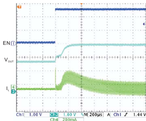
Start-Up Waveform
