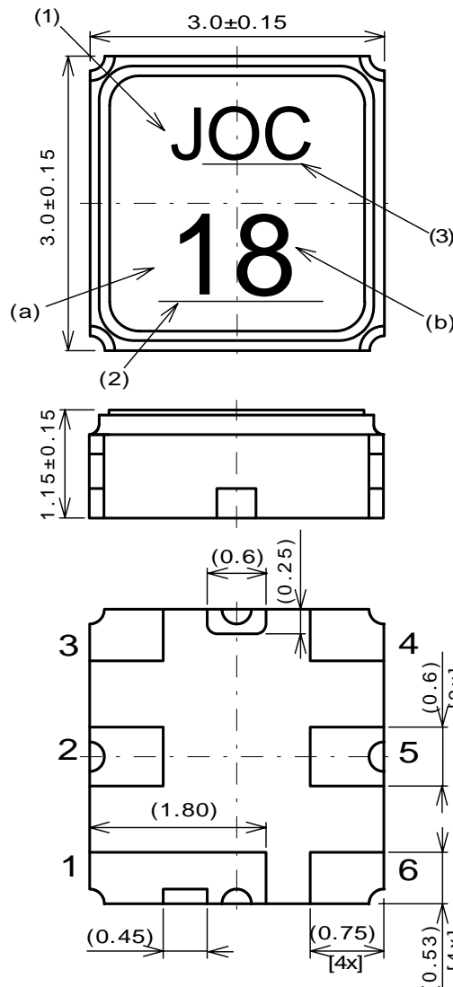
Fig.2 Package dimensions (in mm)
