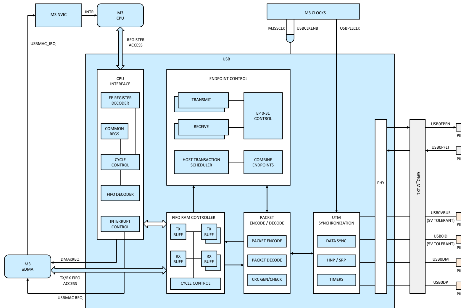
Figure 6-13. USB
