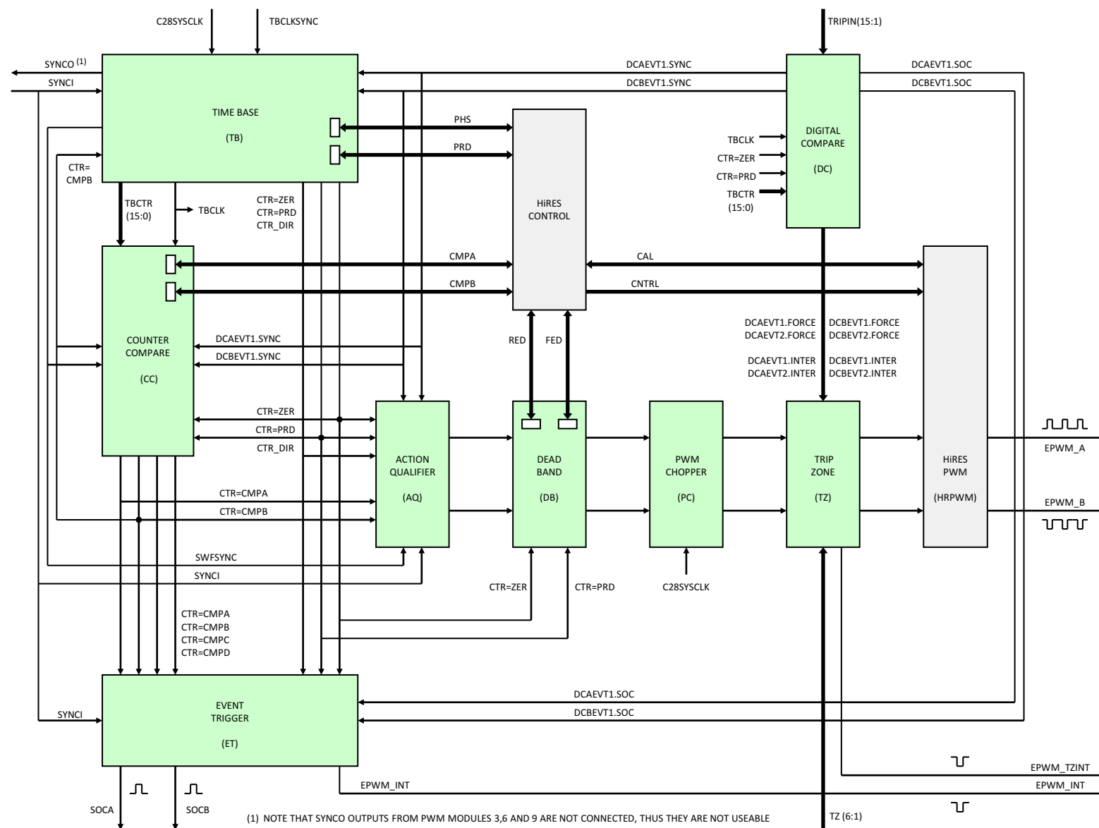
Figure 6-16. Internal Structure of PWM
