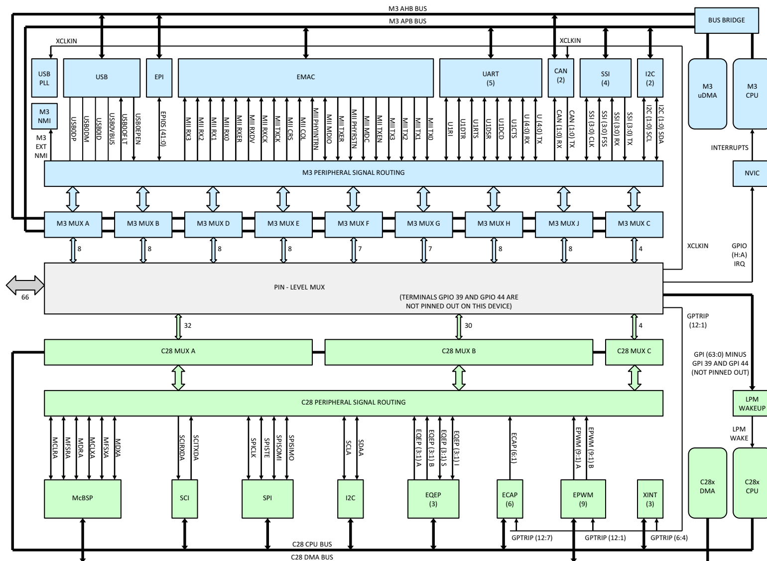
Figure 2-14. GPIO_MUX1 Block
