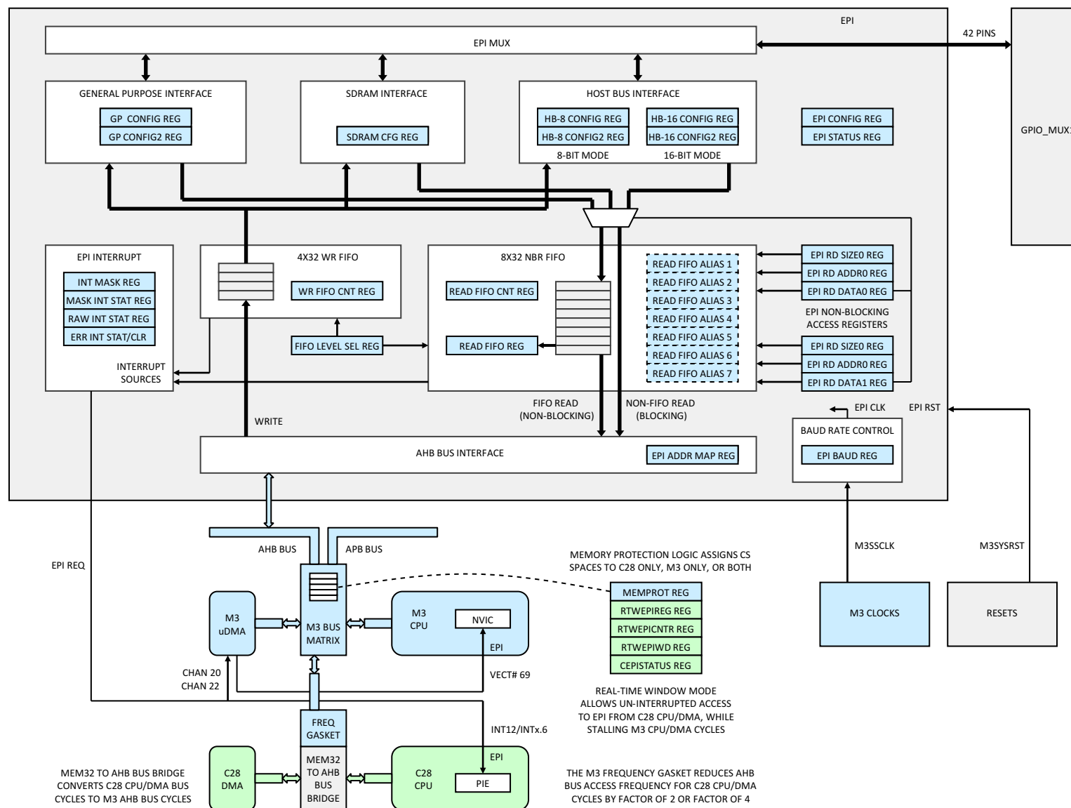
Figure 6-4. External Peripheral Interface (EPI)
