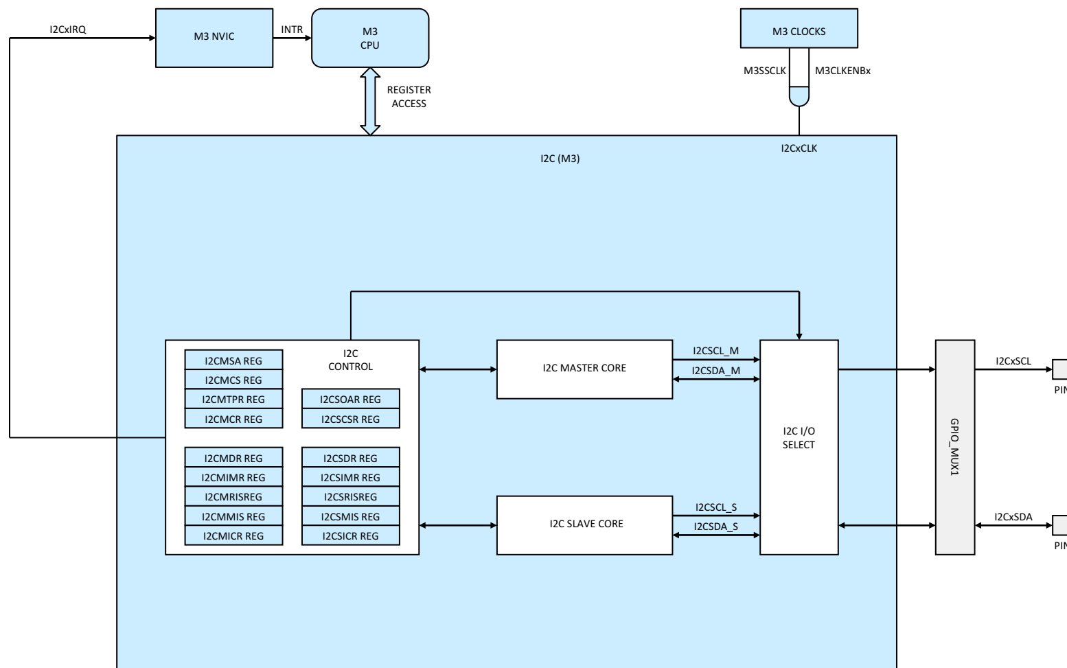
Figure 6-11. I2C (Cortex™-M3)
