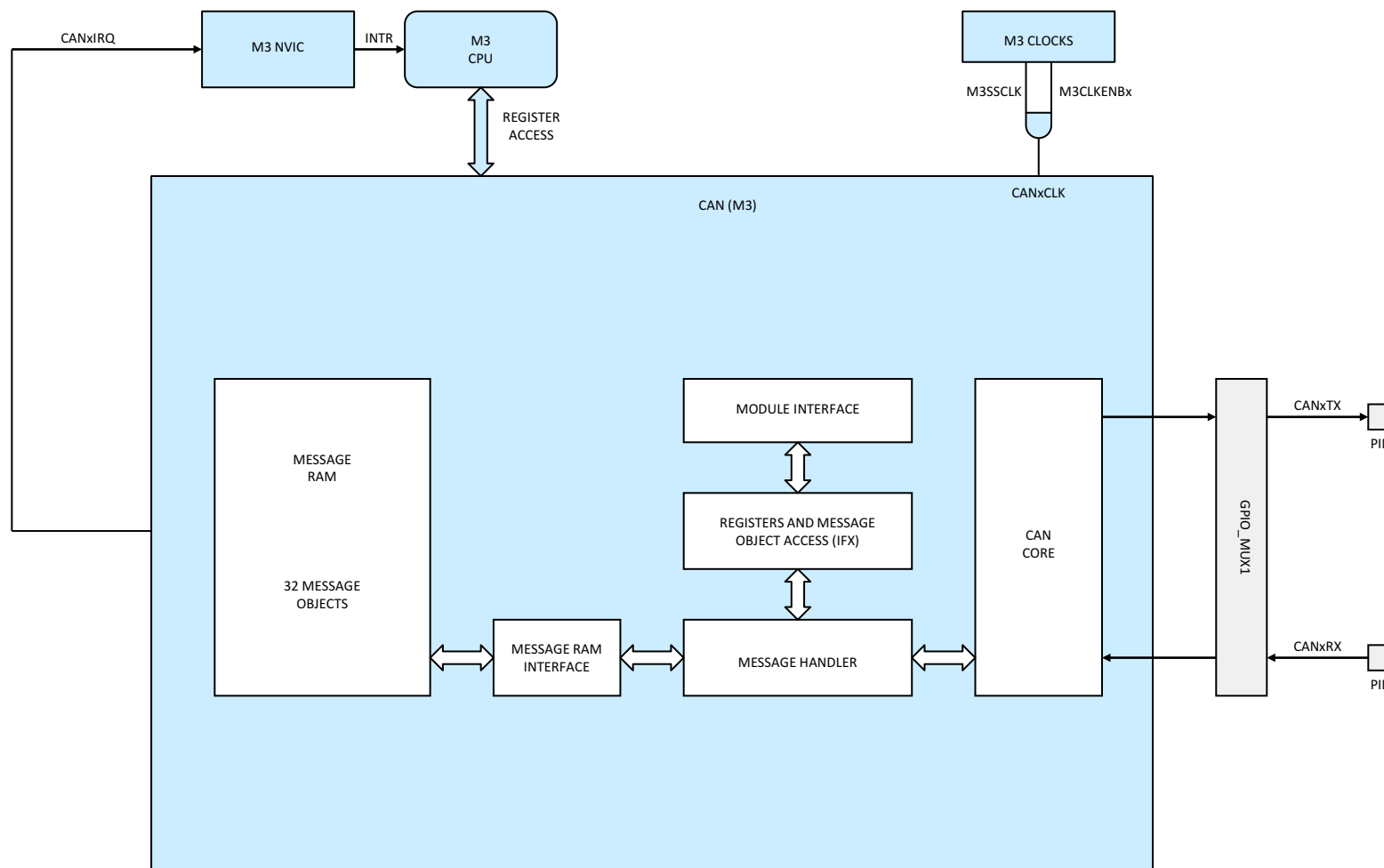
Figure 6-12. CAN (Cortex™-M3)
