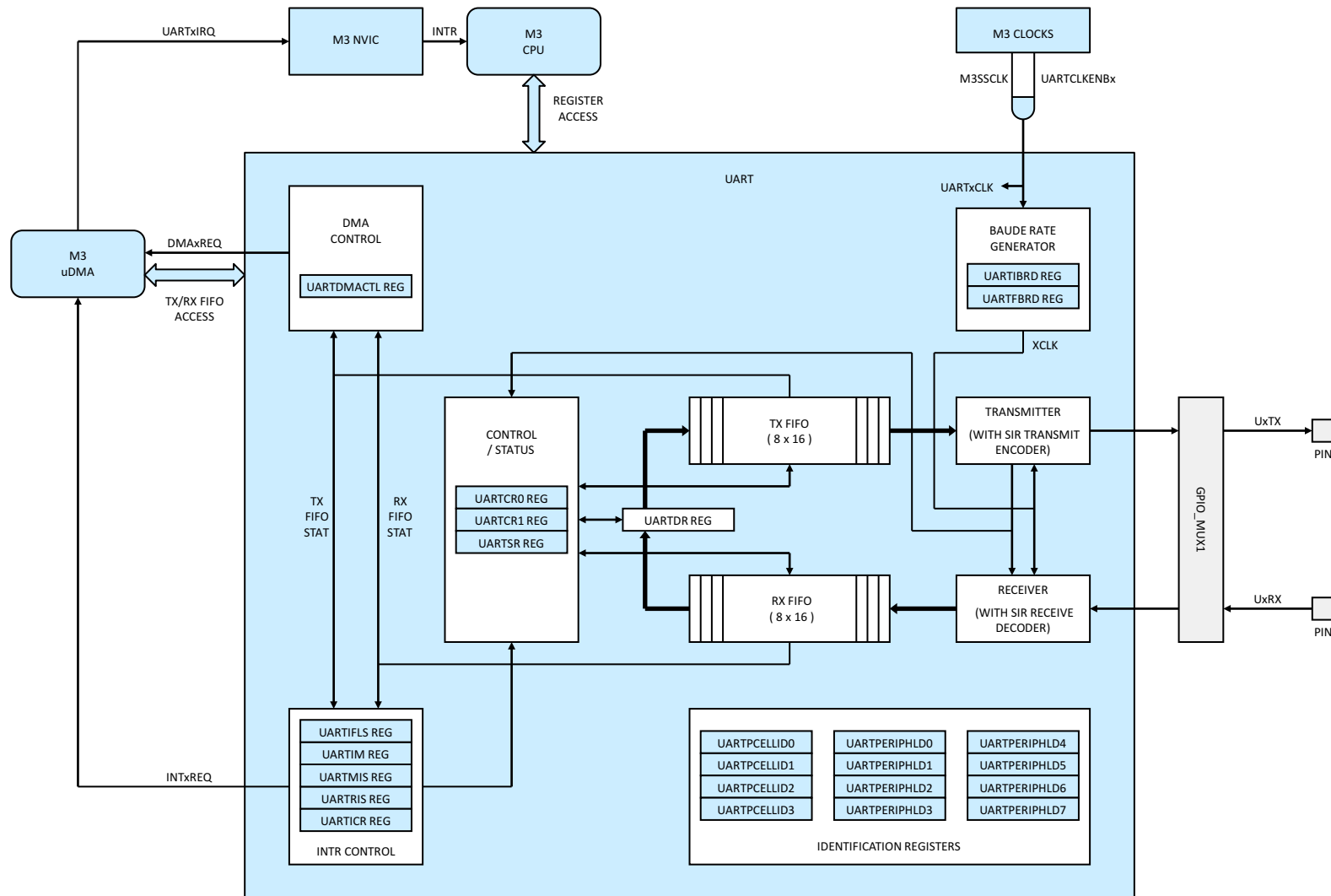
Figure 6-10. UART
