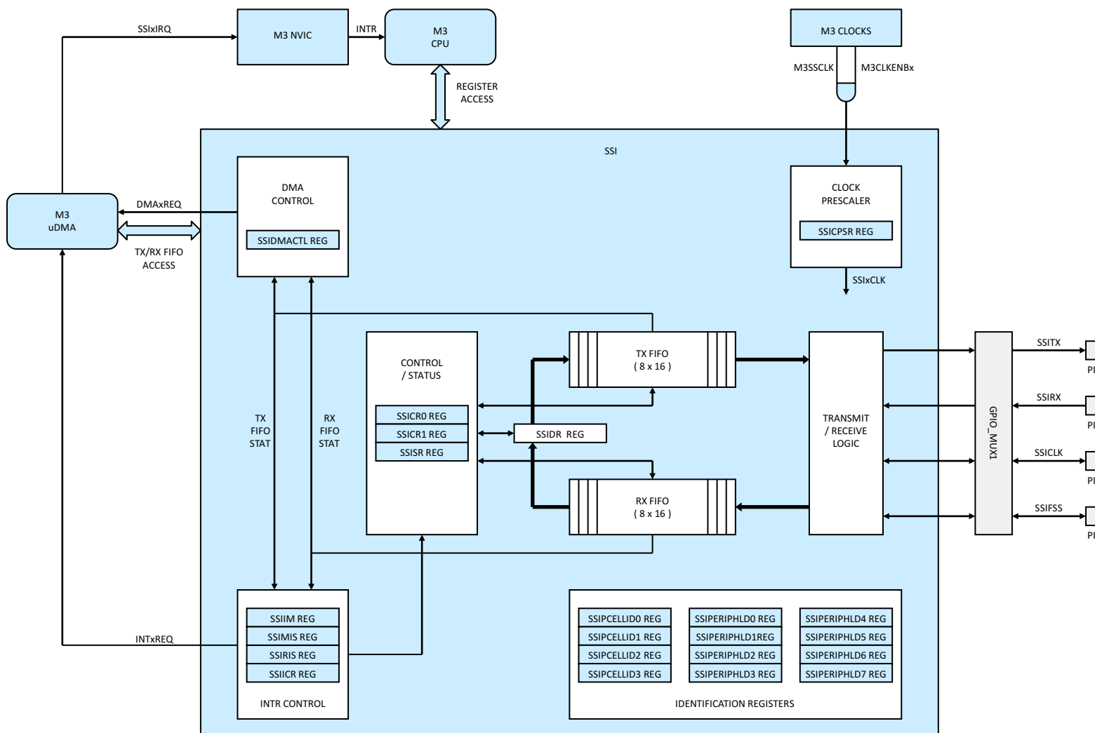
Figure 6-9. SSI
