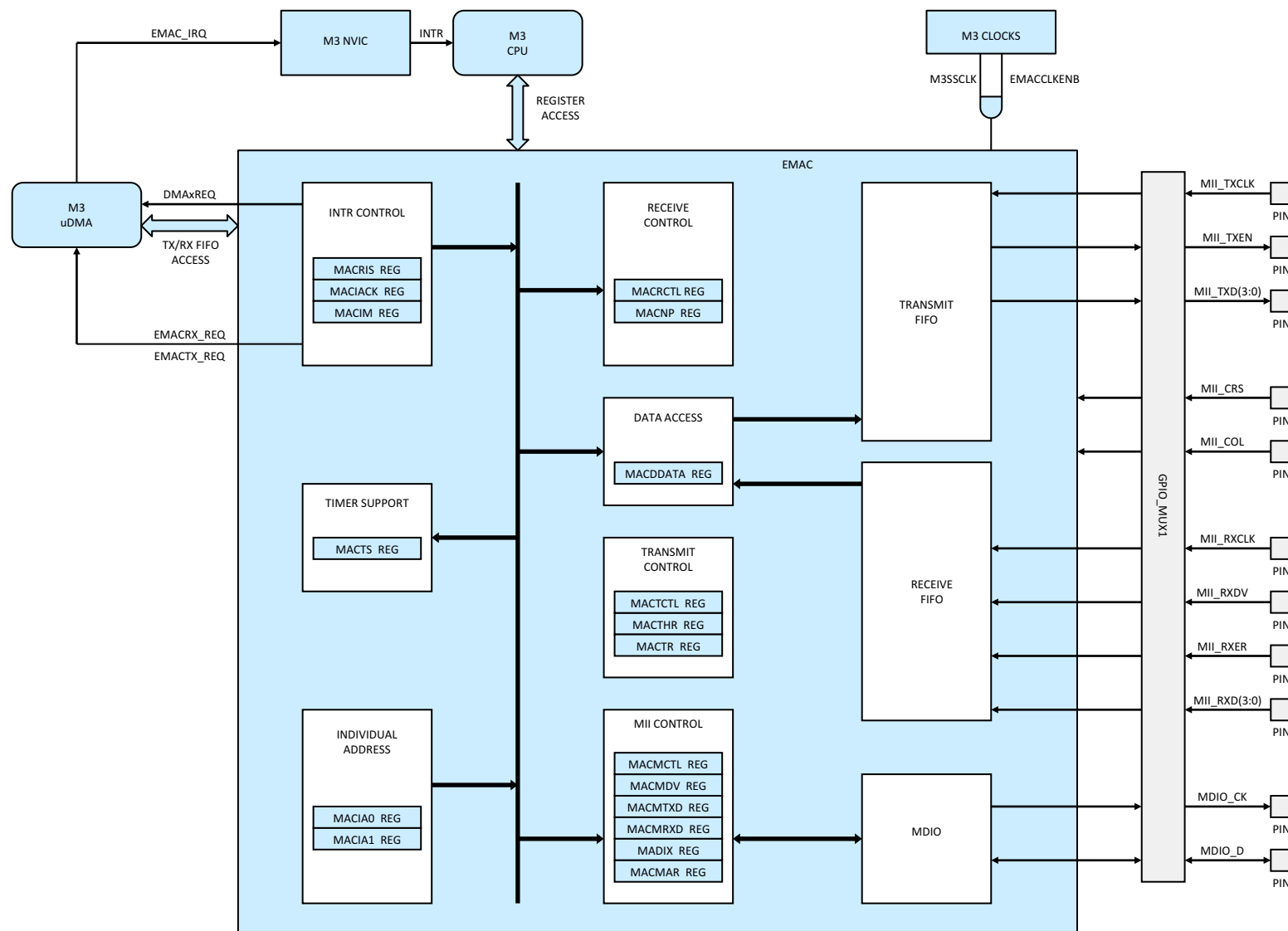
Figure 6-14. EMAC
