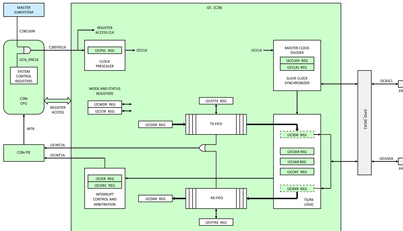
Figure 6-19. I2C (C28x)
