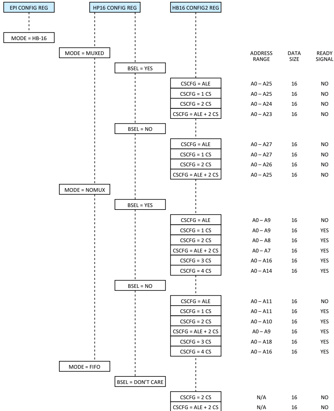
Figure 6-8. EPI 16-Bit Host Bus Mode
