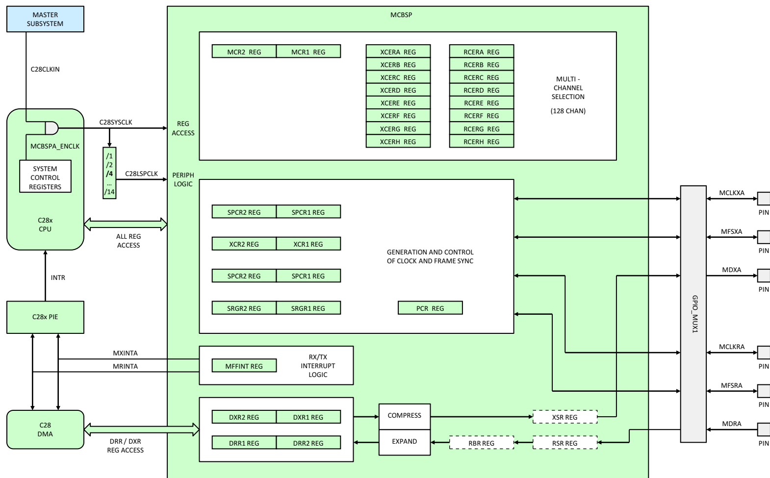
Figure 6-22. McBSP (C28x)
