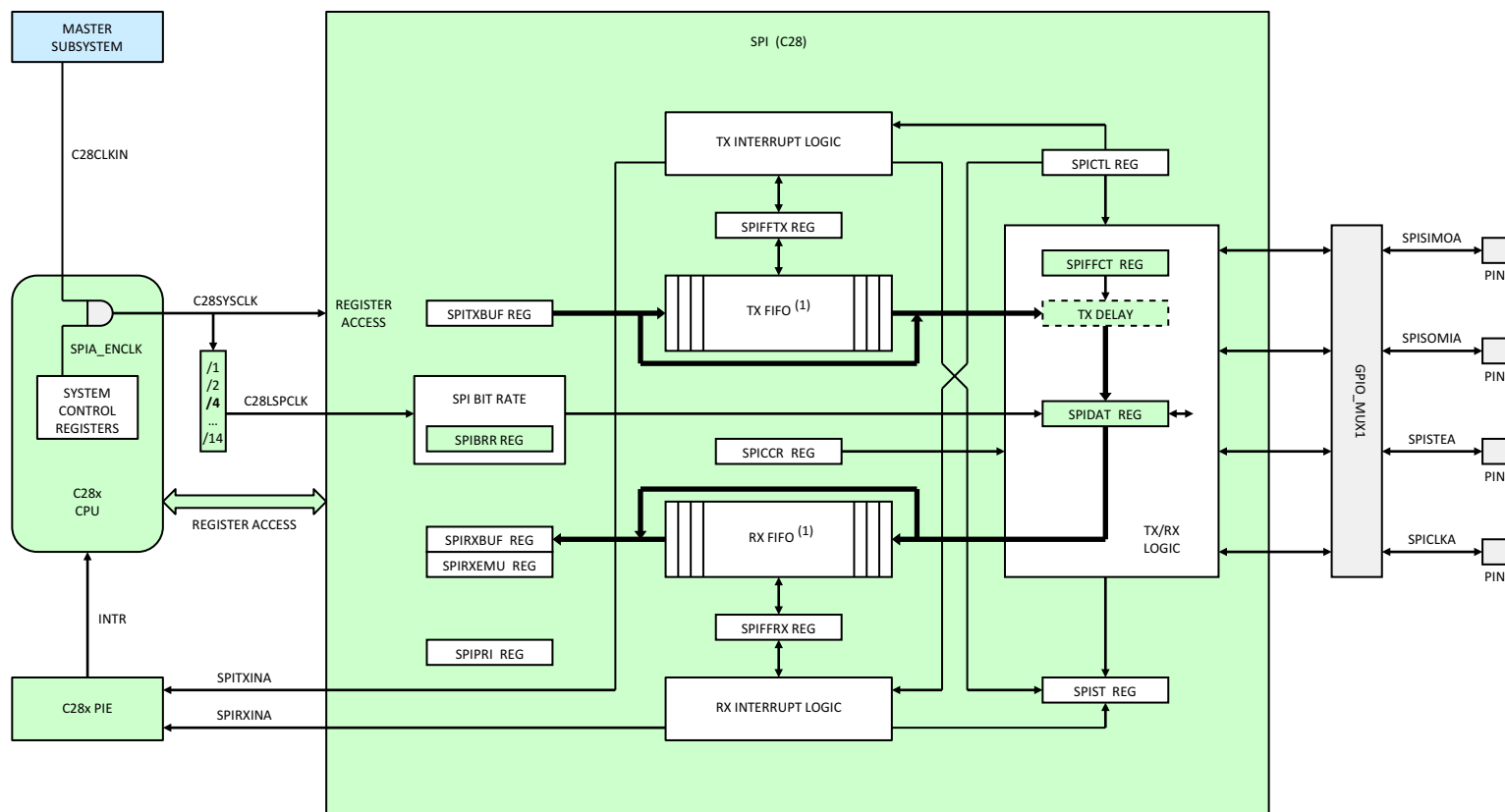
Figure 6-21. SPI (C28x)
