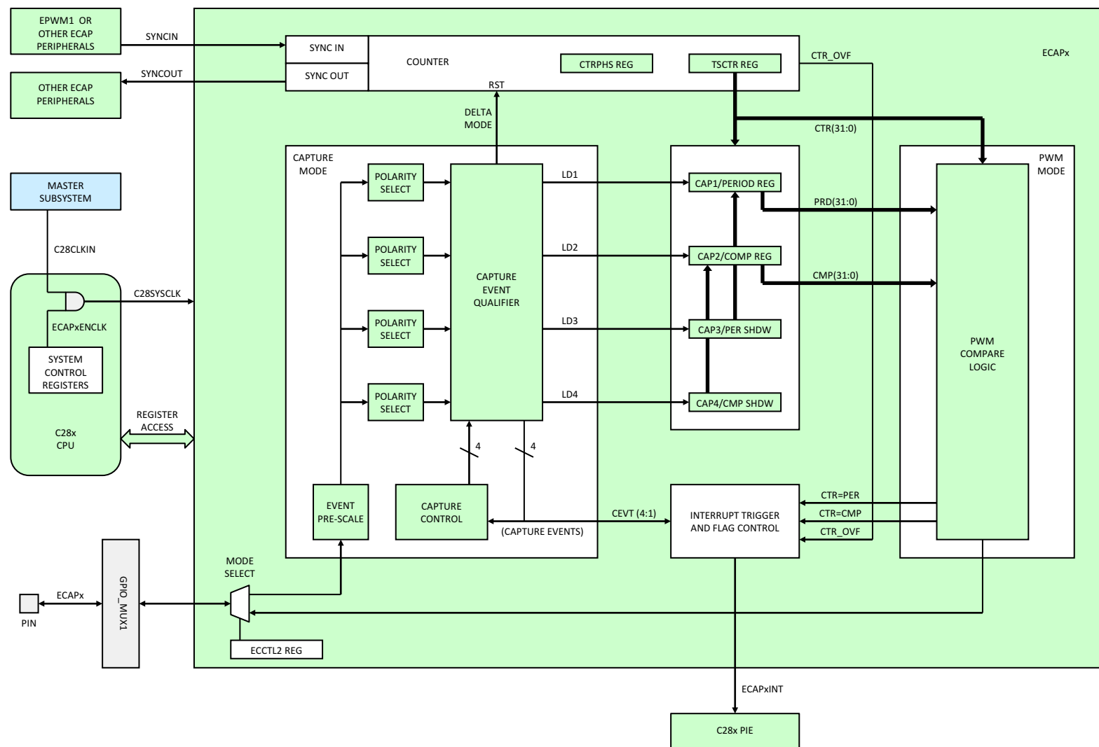
Figure 6-17. eCAP
