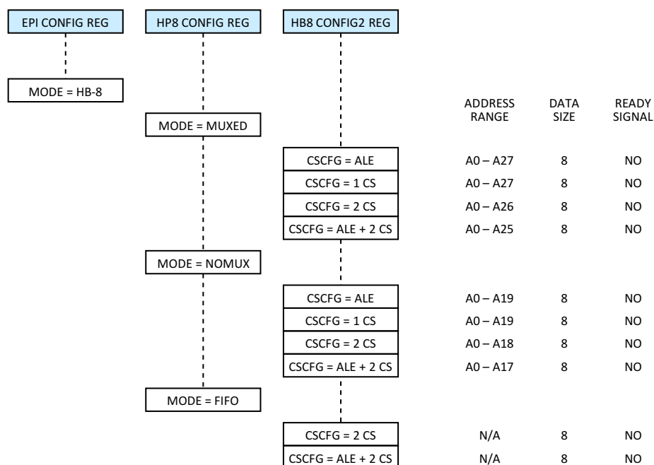
Figure 6-7. EPI 8-Bit Host Bus Mode
