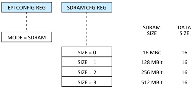
Figure 6-6. EPI SDRAM Mode
