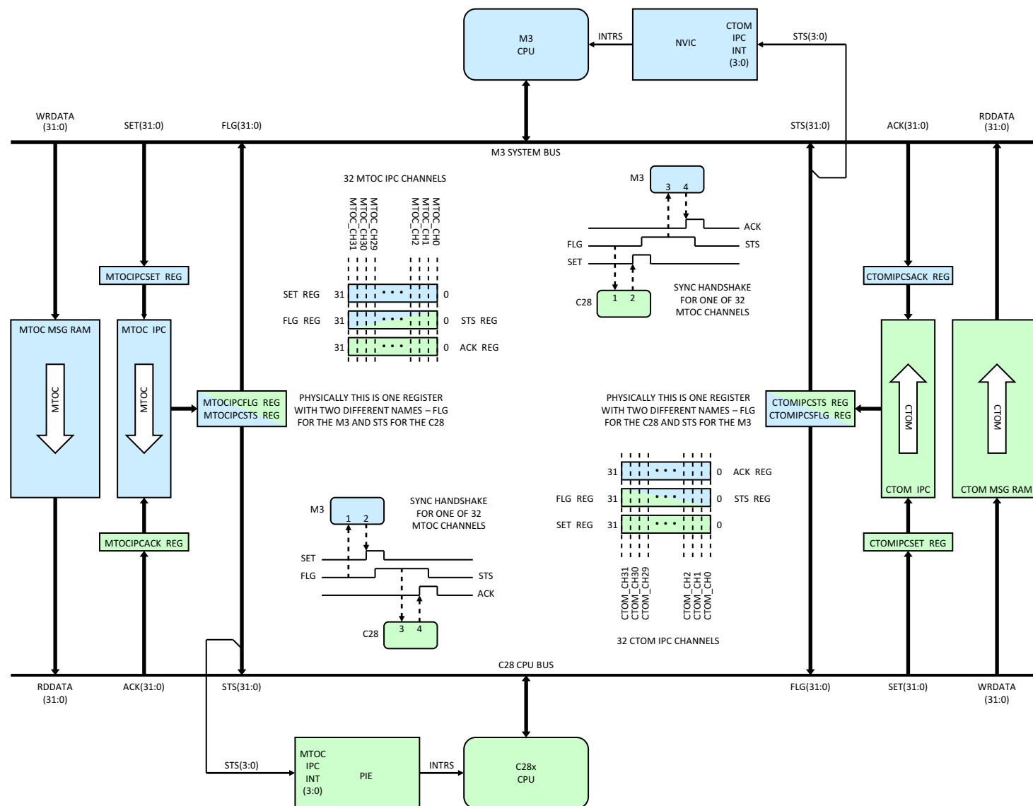
Figure 6-3. Interprocessor Communications (IPC)
