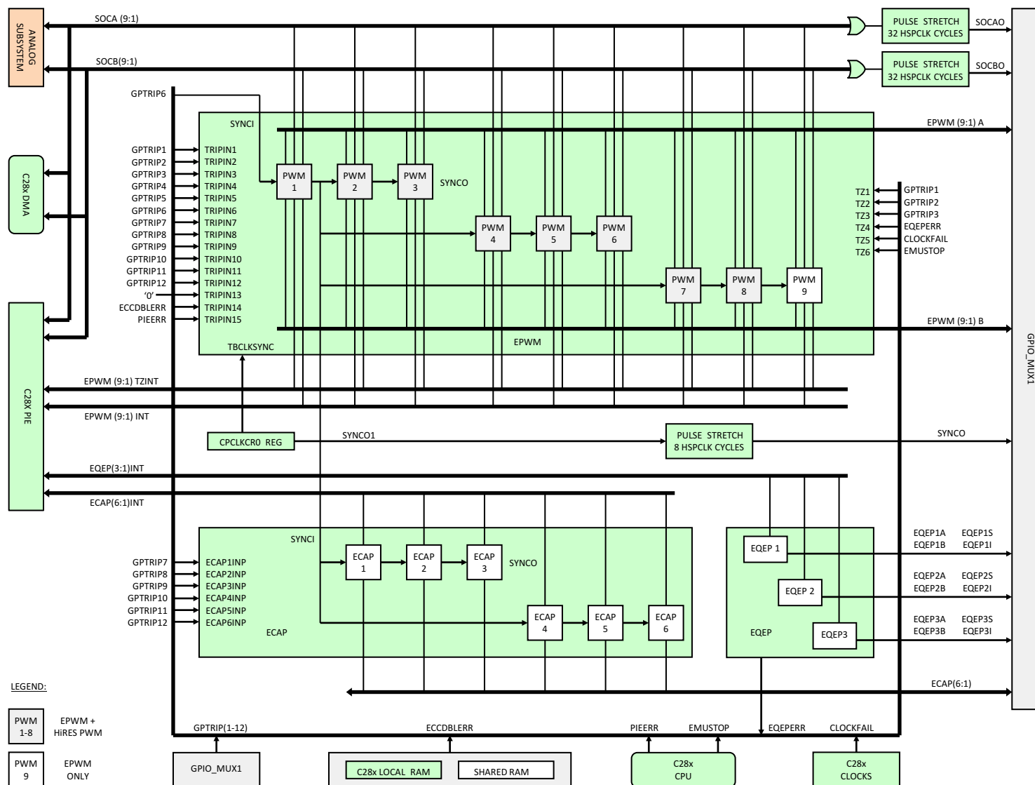
Figure 6-15. PWM, eCAP, eQEP
