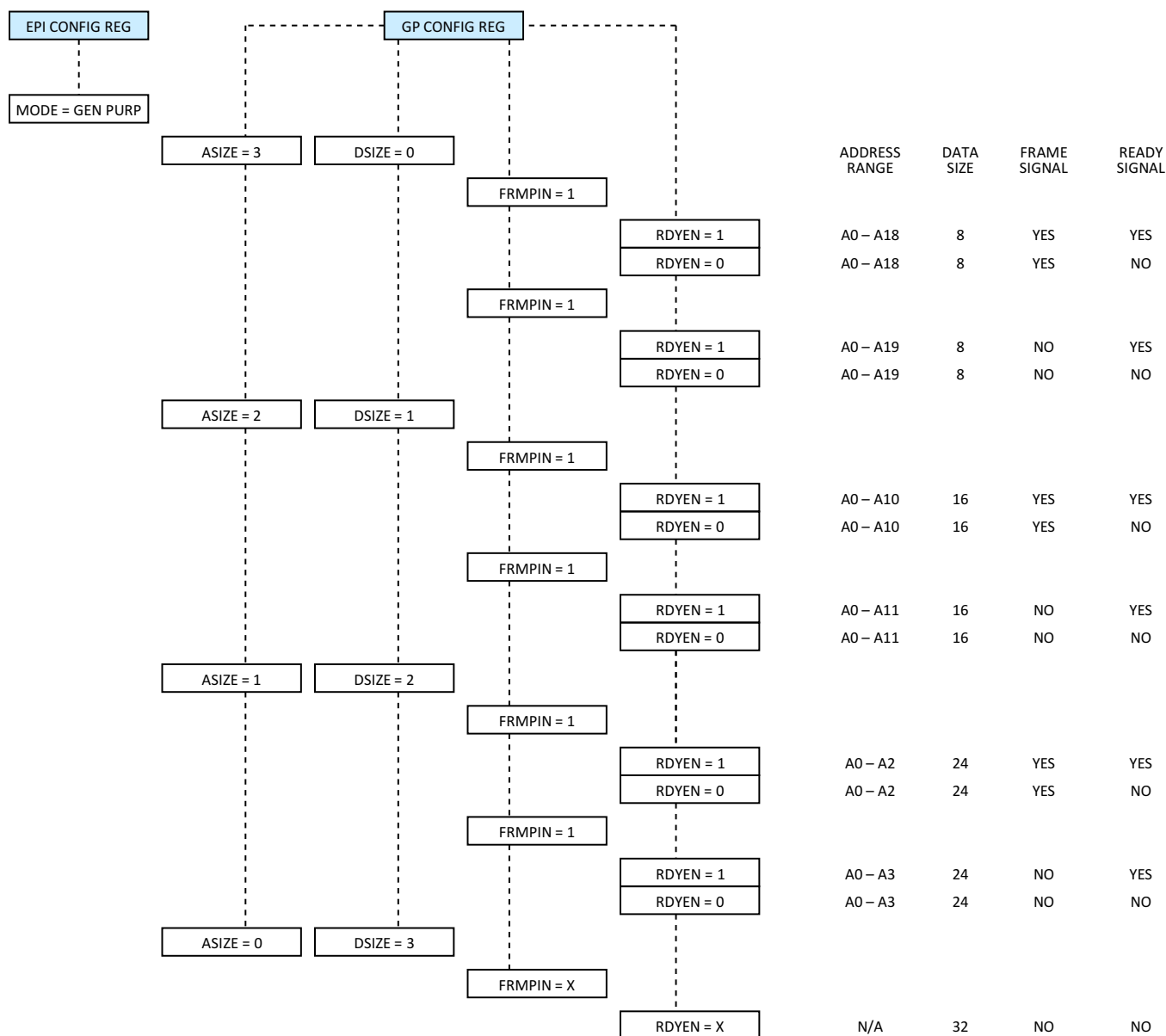
Figure 6-5. EPI General-Purpose Modes
