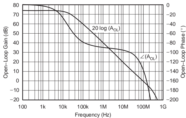
OPEN-LOOP GAIN AND PHASE
