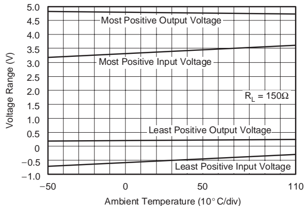
VOLTAGE RANGES vs TEMPERATURE
